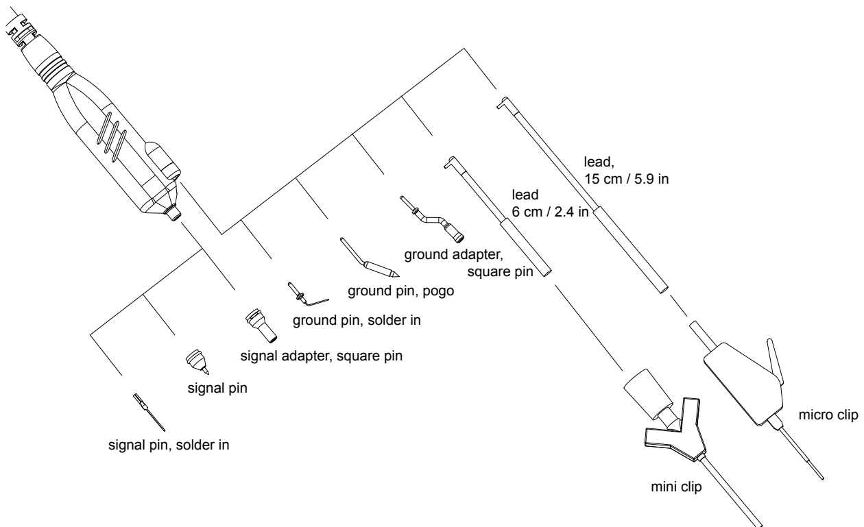
Fig. 1-1: Available accessories
