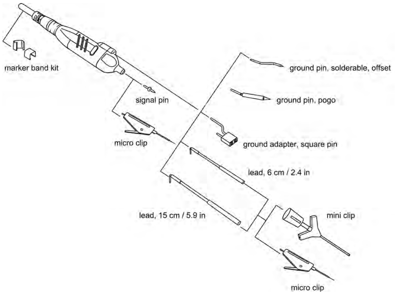
Fig. 1-1: Available accessories
