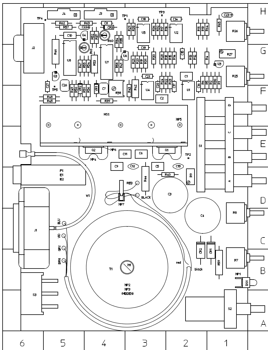
Power and Control Board Component Locator
