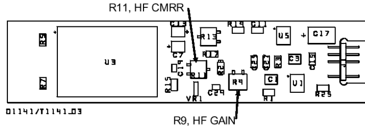
R11, HF CMRR Adjustment
