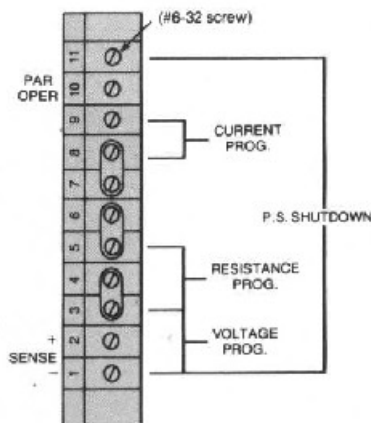
CASE III & IV REAR TERMINAL DETAILS
