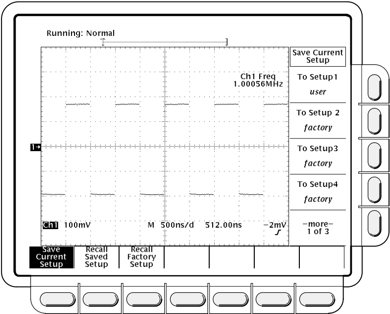
Figure 1-19: Save/Recall Setup Menu
