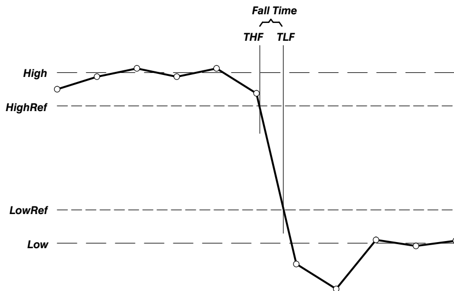
Figure C-2: Fall Time
