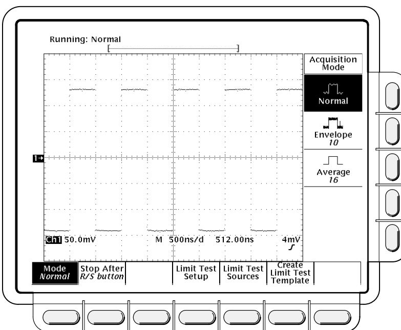
Figure 3-2: Acquire Menu
