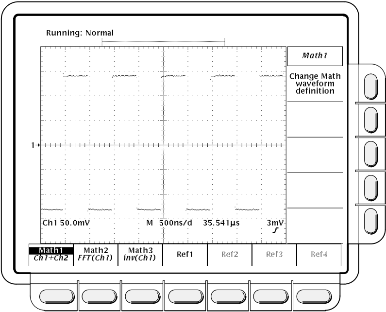
Figure 3-53: More Menu
