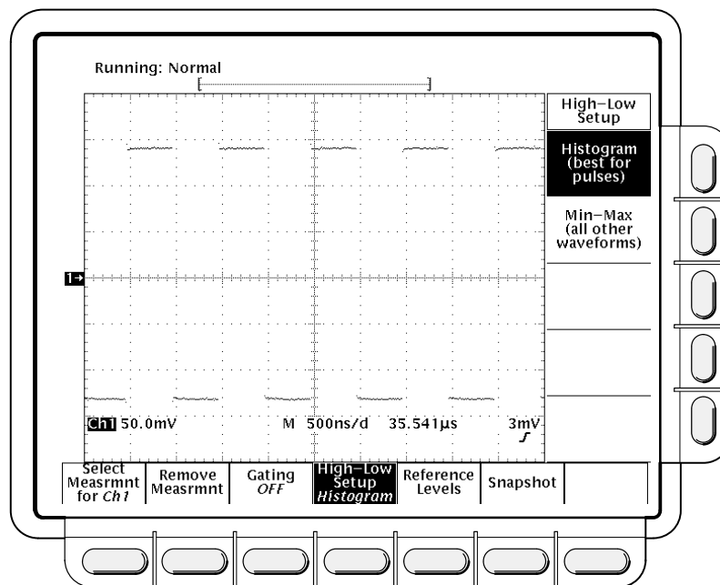
Figure 3-35: Measure Menu—High-Low Setup
