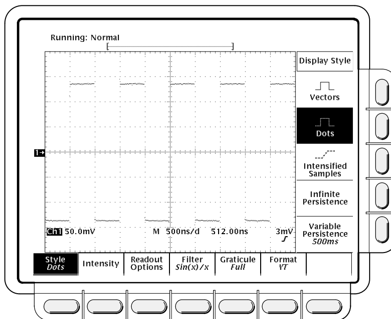
Figure 3-10: Display Menu—Style
