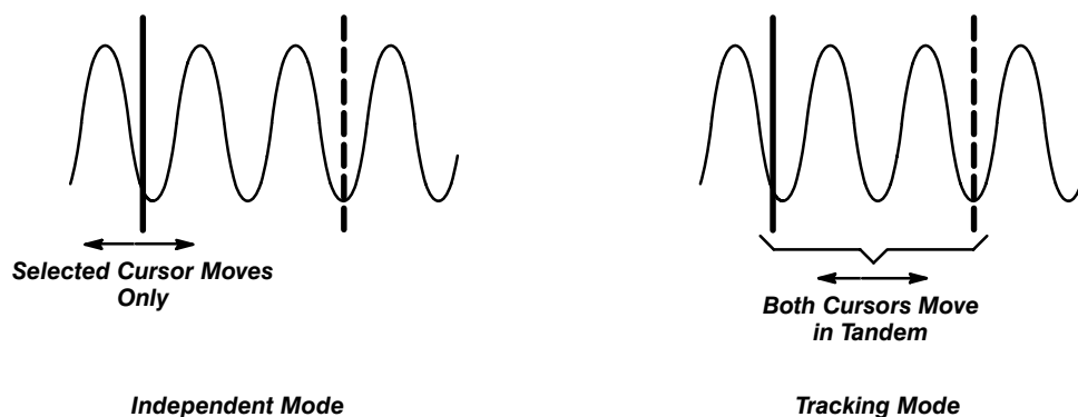
Figure 2-15: Cursor Modes
