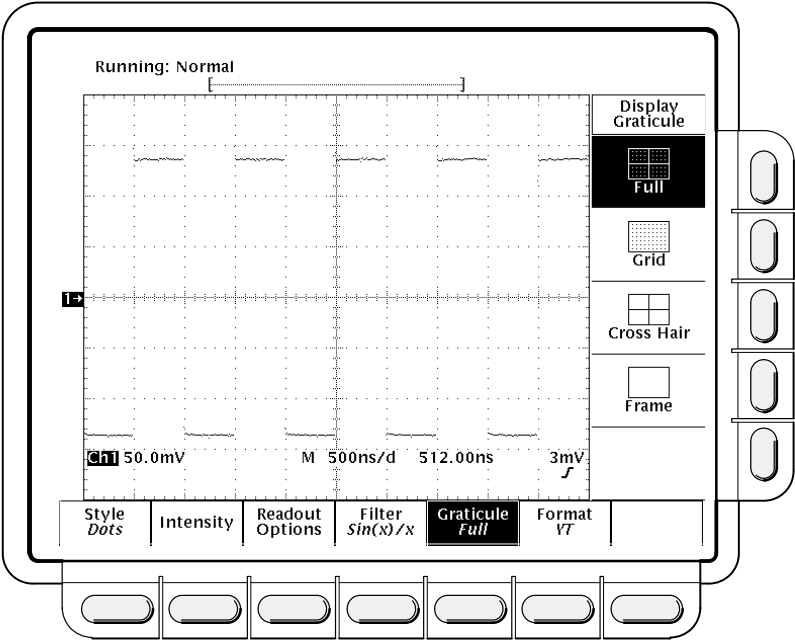
Figure 3-13: Display Menu—Graticule
