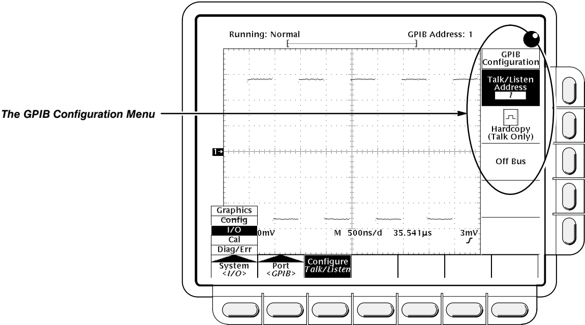
Figure 3-50: Utility Menu
