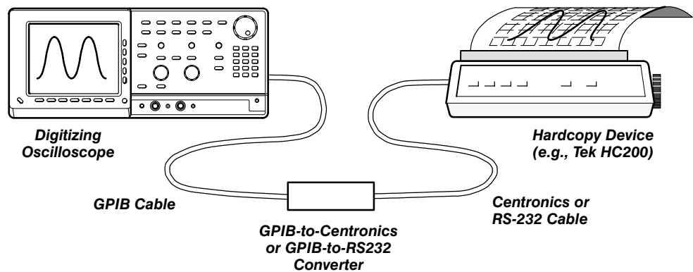
Figure 3-22: Connecting the TDS and Hardcopy Device Via a Converter
