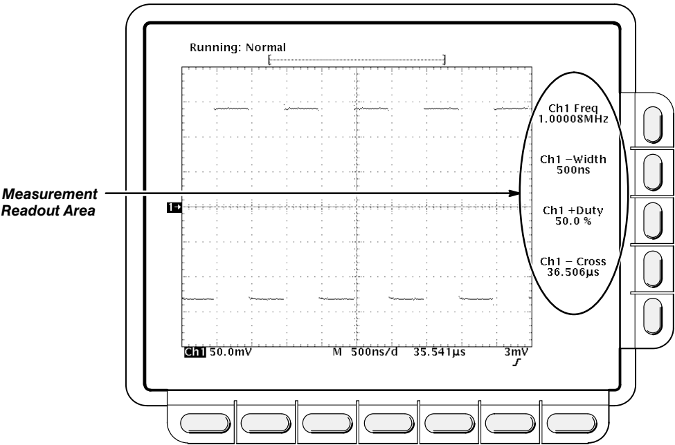
Figure 3-32: Measurement Readouts
