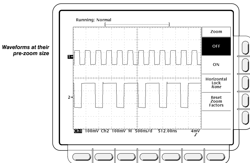
Figure 3-72: Zoom Menu
