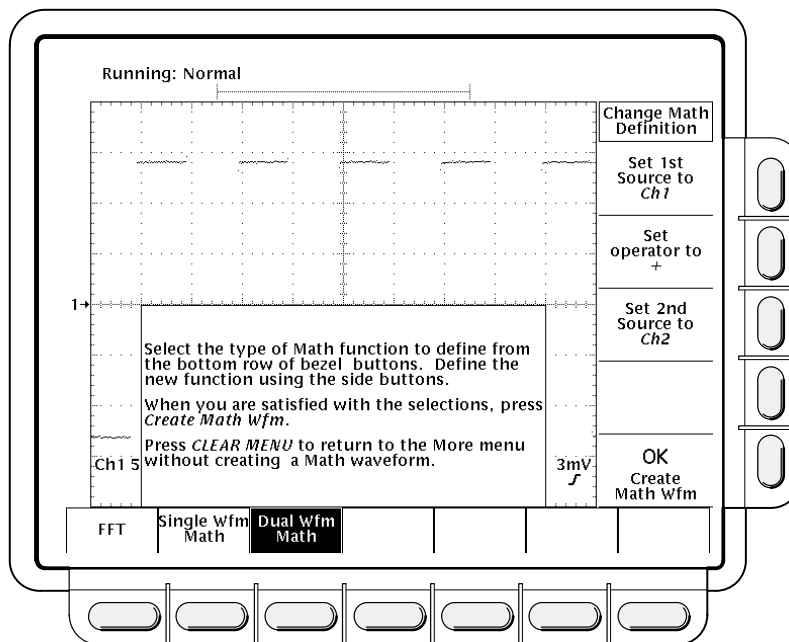
Figure 3-71: Dual Waveform Math Main and Side Menus
