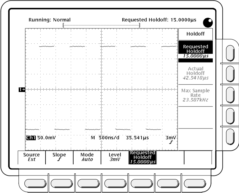
Figure 3-66: Trigger Menu—Holdoff
