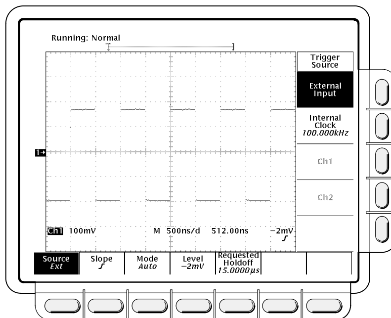
Figure 3-63: Trigger Menu
