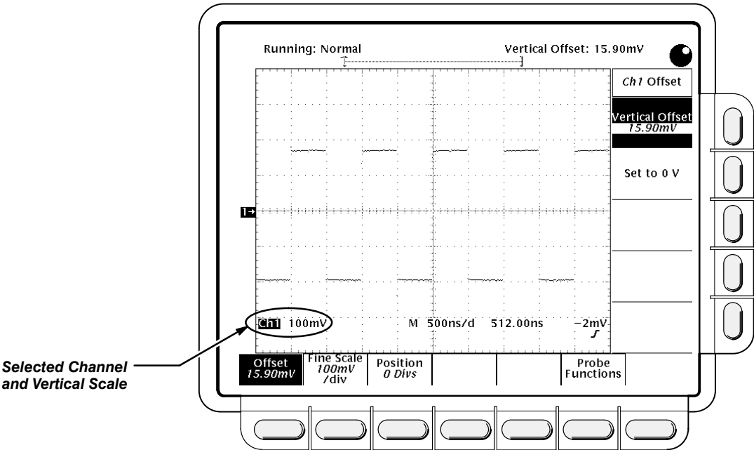
Figure 3-68: Vertical Readouts
