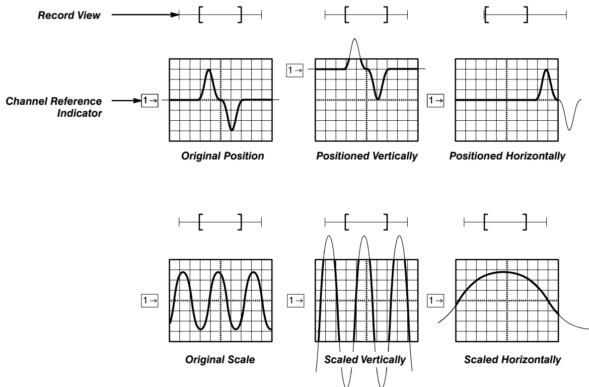
Figure 2-11: Scaling and Positioning
