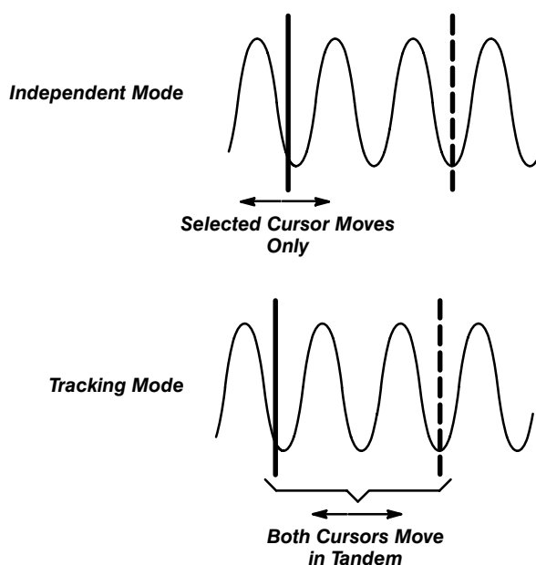
Figure 3-5: Cursor Modes
