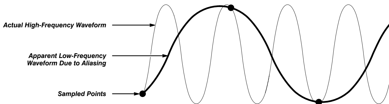
Figure 2-12: Aliasing
