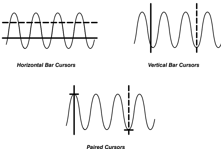
Figure 2-14: Cursor Types
