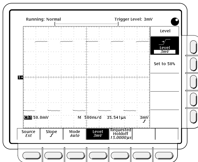
Figure 3-65: Trigger Menu—Level
