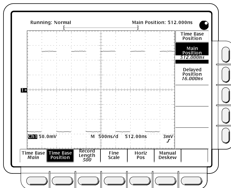
Figure 3-28: Horizontal Menu—Time Base Position
