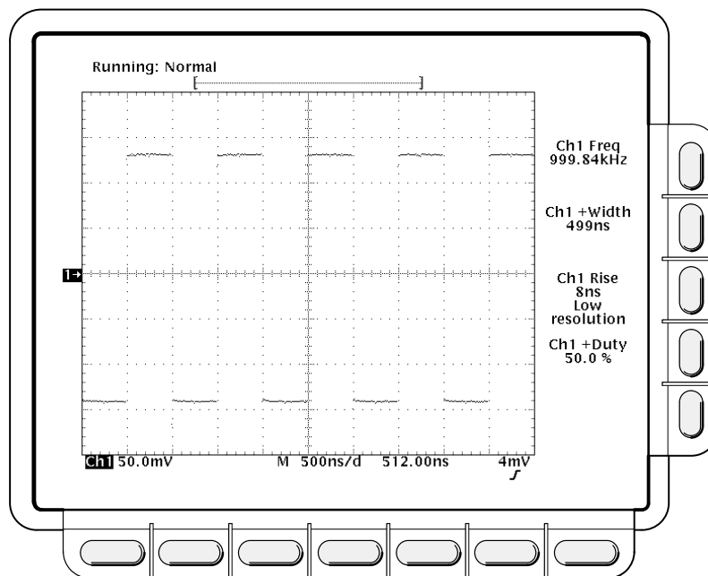
Figure 1-17: Four Simultaneous Measurement Readouts
