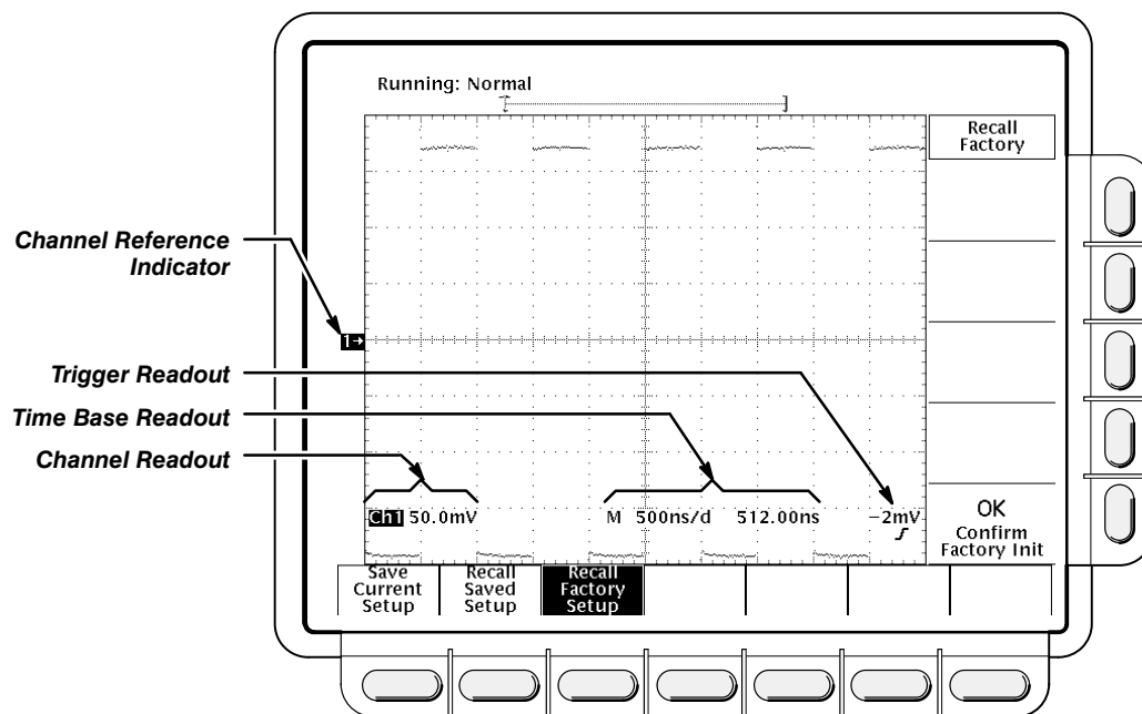
Figure 1-9: Display Elements
