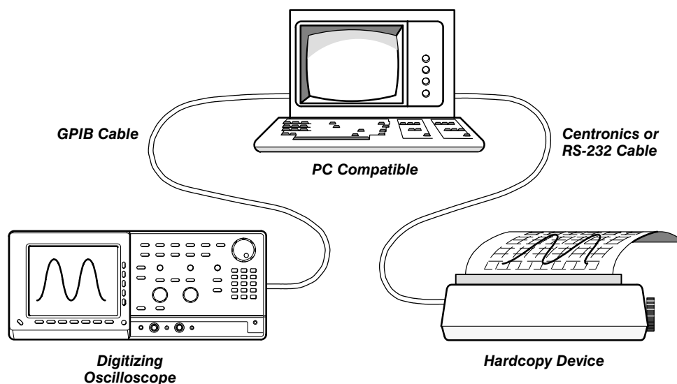
Figure 3-23: Connecting the TDS and Hardcopy Device Via a PC
