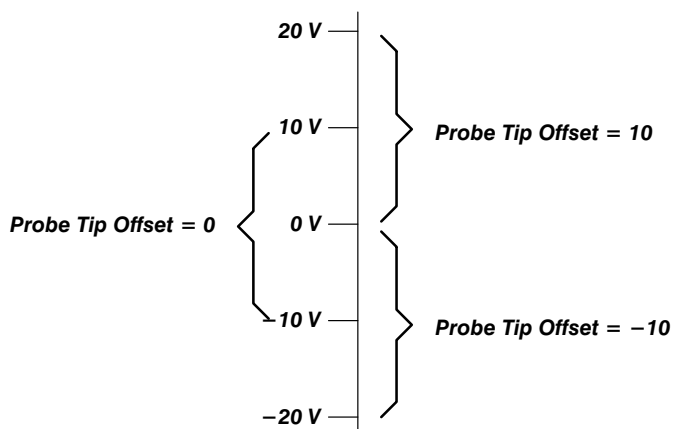
Figure 3-43: Probe Tip Offset and Dynamic Range
