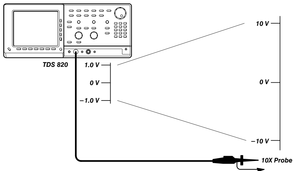
Figure 3-42: TDS 820 Vertical Scale and Probe Attenuation Factor
