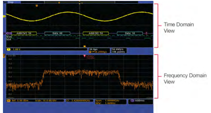
The upper half of the MDO4000 Series display shows the Time Domain view of the analog and digital channels, while the lower half shows the Frequency Domain view of the RF channel. The orange bar – Spectrum Time – shows the period of time used to calculate the RF spectrum.
