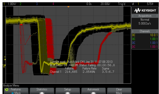
Limit testing made easy with the "automask" feature.
