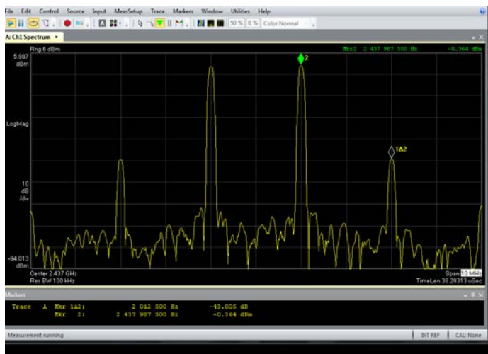
Using data acquired from the V-Series, VSA shows an excellent third order intercept (TOI) value of 26 dBm.
