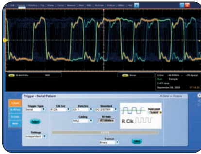
► Serial pattern triggering to debug pattern-dependent issues.
