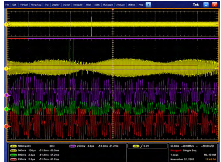
Zoom in on four areas of interest simultaneously to compare them
