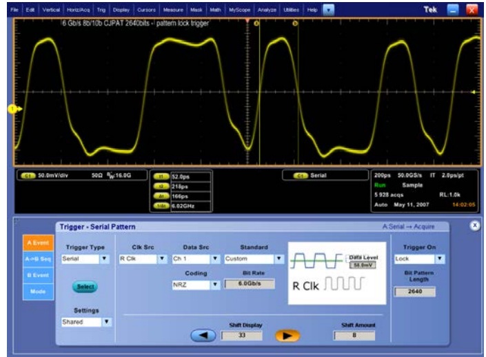
NRZ Pattern Lock Triggering of a 640-bit long SATA serial pattern at 6 Gbps
