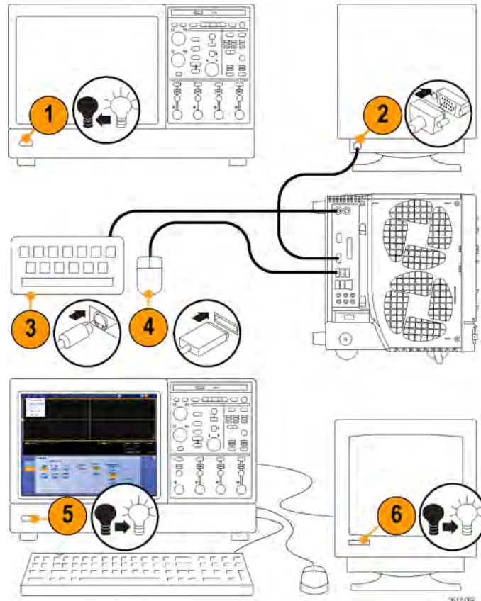
DPO7000C Series
