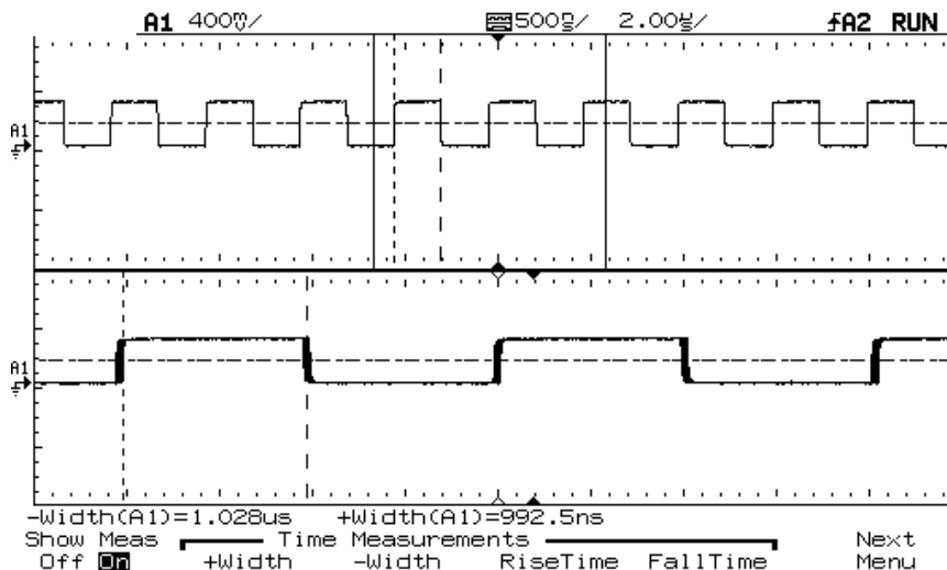
Isolating Event for Frequency Measurement
