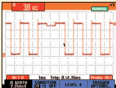
Pulse width triggering allows you to find anomalies like missing pulses
