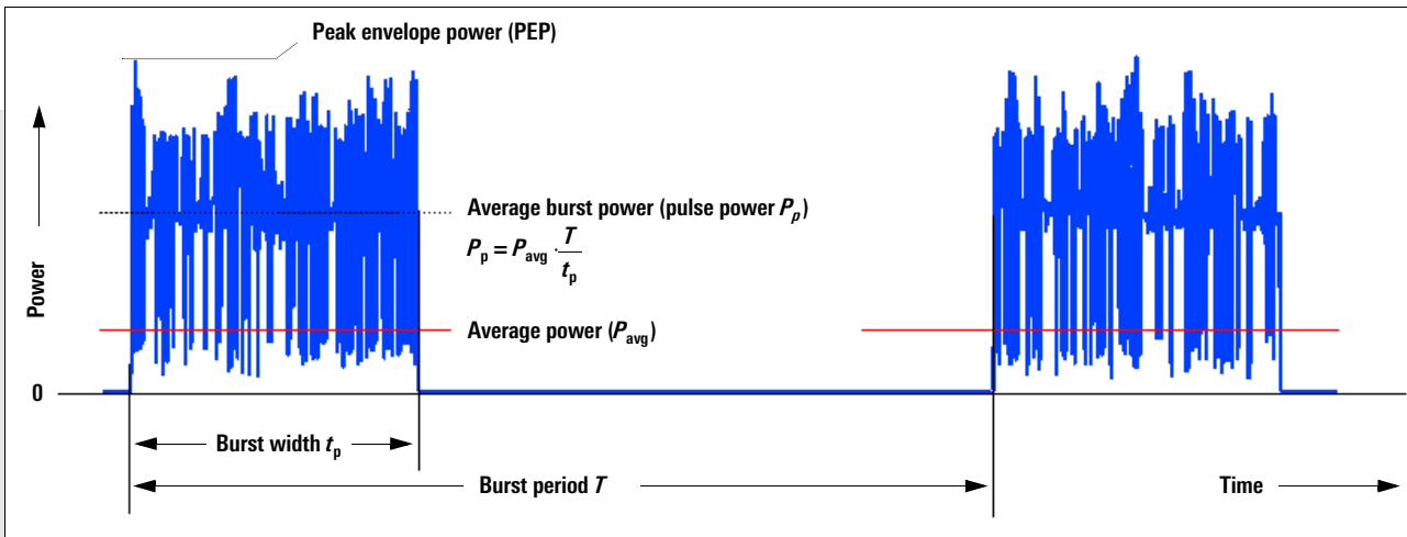
Definition of the main power parameters using the transmitter signal of an NADC mobile station as an example; the average burst power can be displayed on the R&S®NRVS, R&S®NRVD and R&S®URV55 base units after entering the duty cycle t_p/T ; required is a sensor that is able to precisely measure the average power P_{avg} , i.e. a thermal sensor or a diode sensor operated in the square-law region
