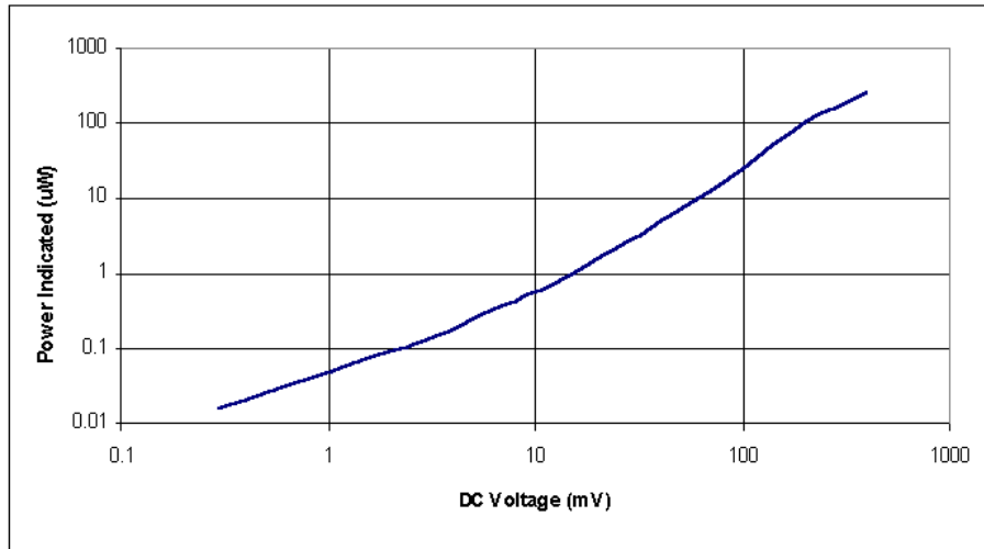
Figure 3-3 Typical Power Error Introduced in an Agilent E9304A power sensor by DC Voltage
