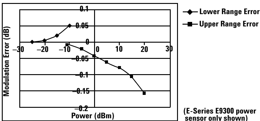
Figure 2-6 Wideband CDMA Error of Agilent E-Series E9300 power sensor versus corrected CW sensor
