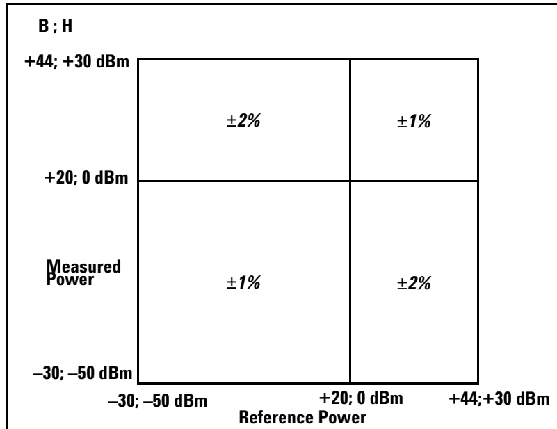
Figure 3-11 Relative Mode Power Measurement Linearity with Agilent EPM power meter at 25 °C ± 10 °C (typical)
