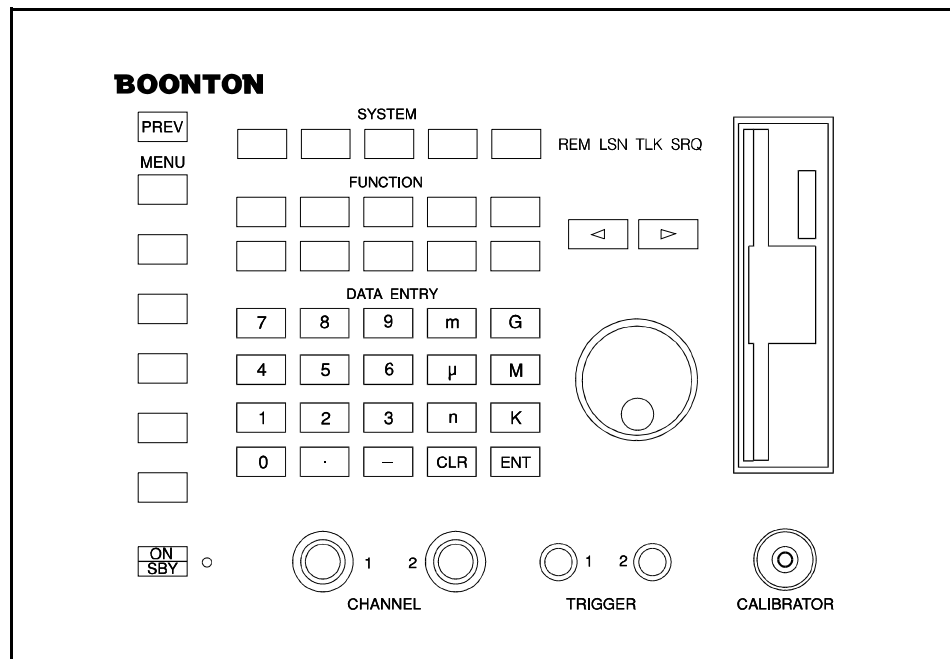
Figure 4-6. Data Entry Keypad
