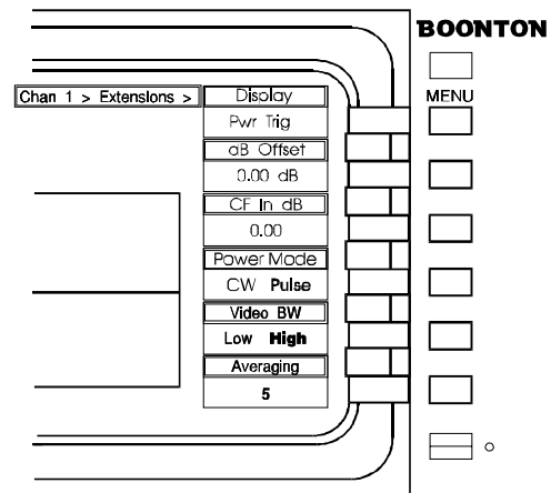
Figure 4-1c. Chan 1 > Extensions > Submenu
