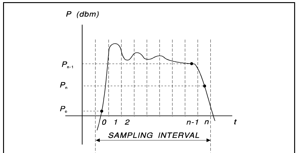
Figure 6-7 Sampling Intervals
