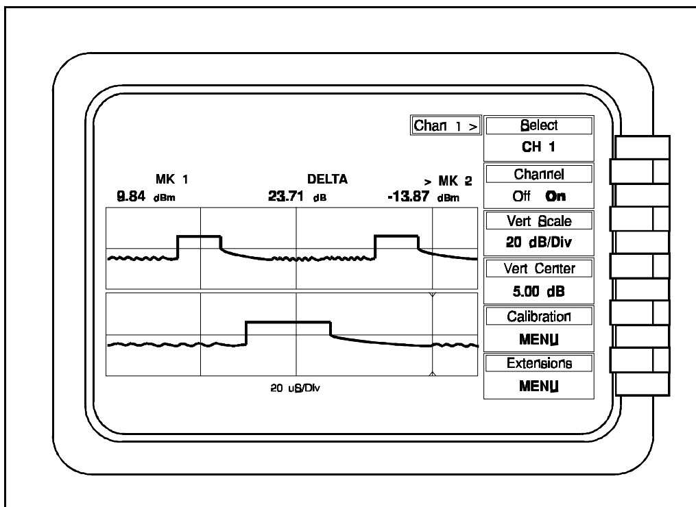
Figure 3-10. Split-Screen Display
