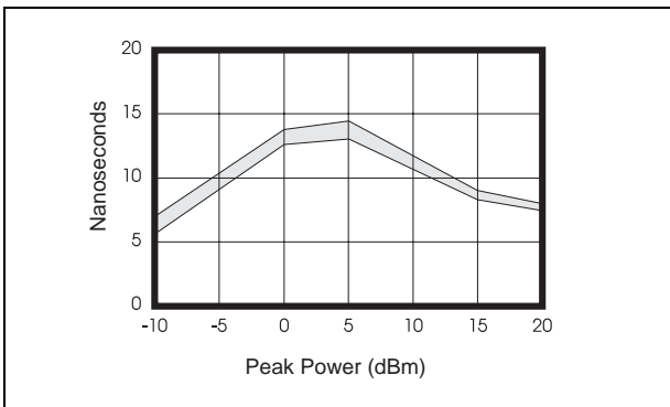
*Typical Risetime in High Bandwidth Mode
