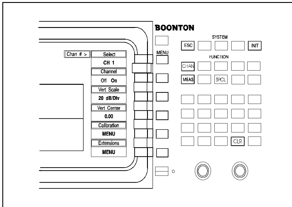
Figure 3-4. Front Panel Controls Used in Calibration Procedures
