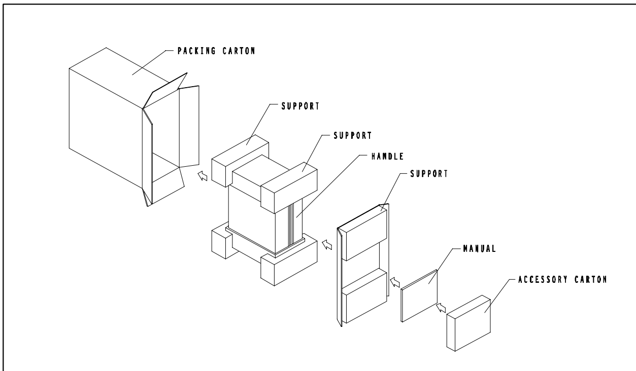
Figure 2-1. Packaging Diagram
