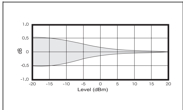
Temperature Influence (±4° from calibration)
