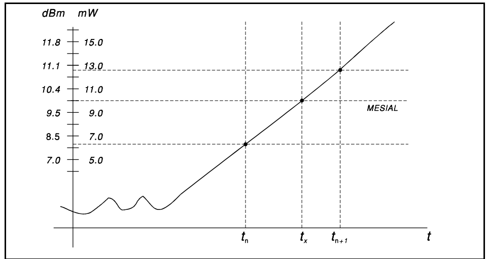
Figure 6-6. Time Interpolation
