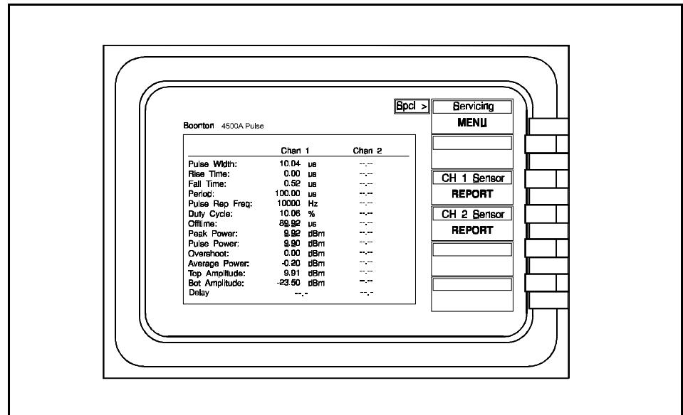
Figure 4-9. Text Mode Display in Power Mode
