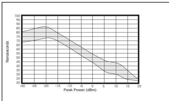
*Typical Risetime in High BW Mode
