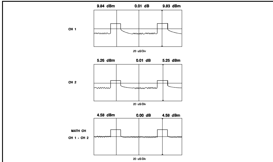
Figure 4-17. Generating a Difference Waveform Using Channel Math
