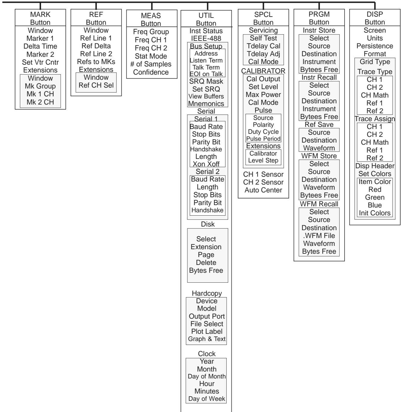
Figure 4-2. Control Menu Structure
