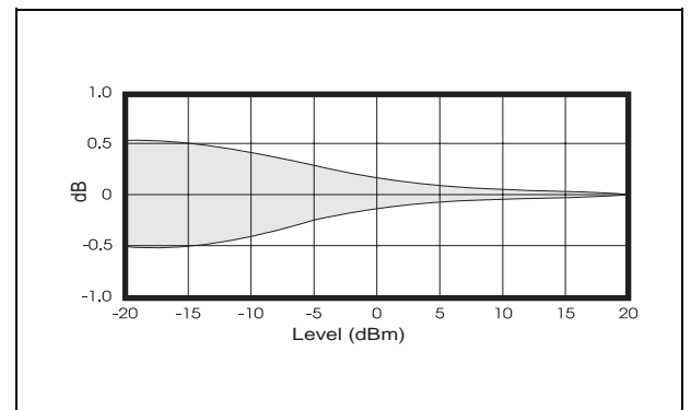
Temperature Influence (±4° from calibration)
