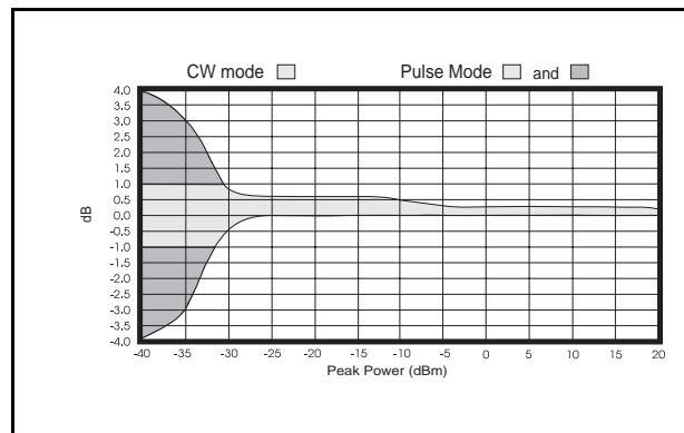
Temperature Influence ( \pm 4^\circ from calibration)
