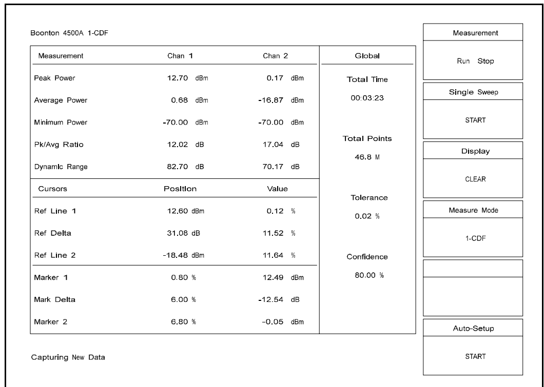
Figure 4-44. Text Mode Display (when in Stat ⇌ mode)
