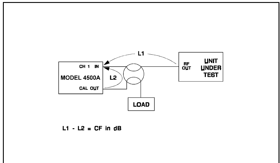
Figure 4-15. Illustration of Measurement (L1) and Calibration (L2) Paths
