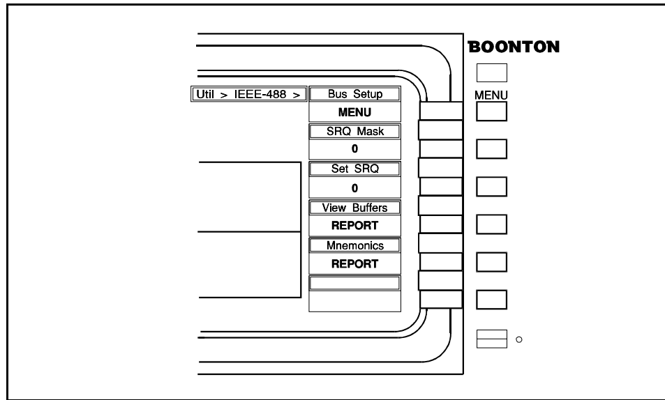
Figure 4-27. Util > IEEE-488 > Submenu
