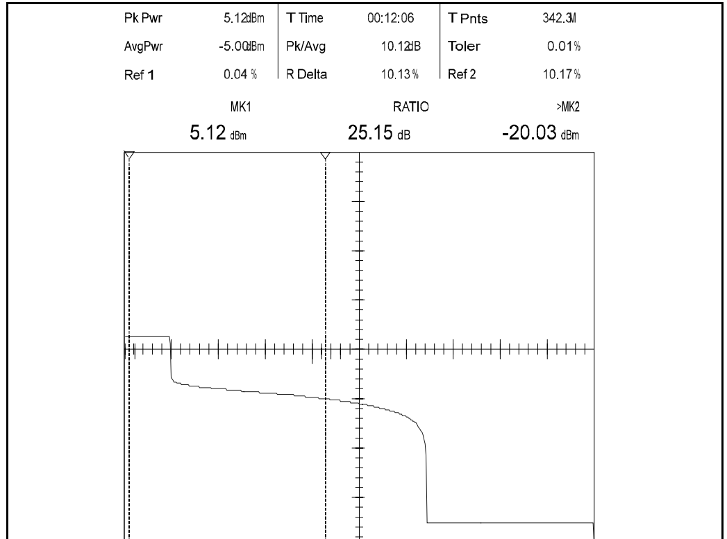
Figure 3-14. 1-CDF Display
