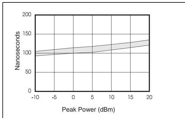
*Typical Risetime in High BW Mode
