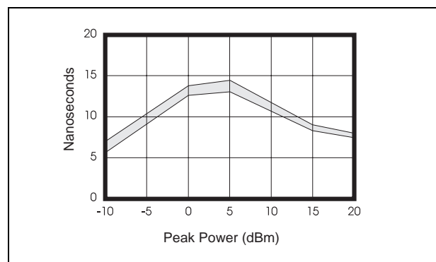
*Typical Risetime in High Bandwidth Mode
