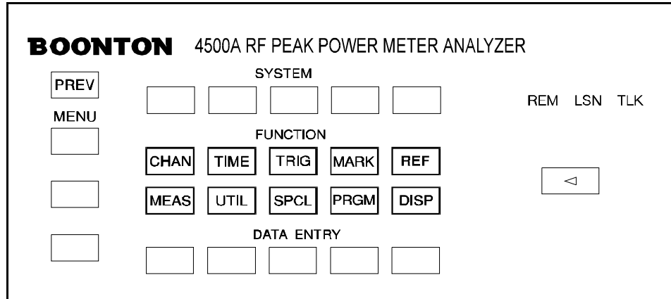
Figure 4-11. Function Keys
