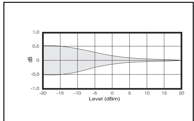
Temperature Influence (±4° from calibration)
