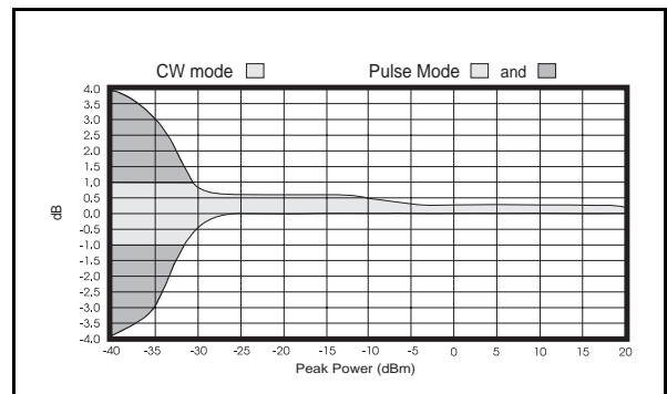
Temperature Influence ( \pm 4^\circ from calibration)
