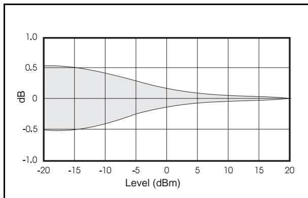
Temperature Influence (±4° from calibration)
