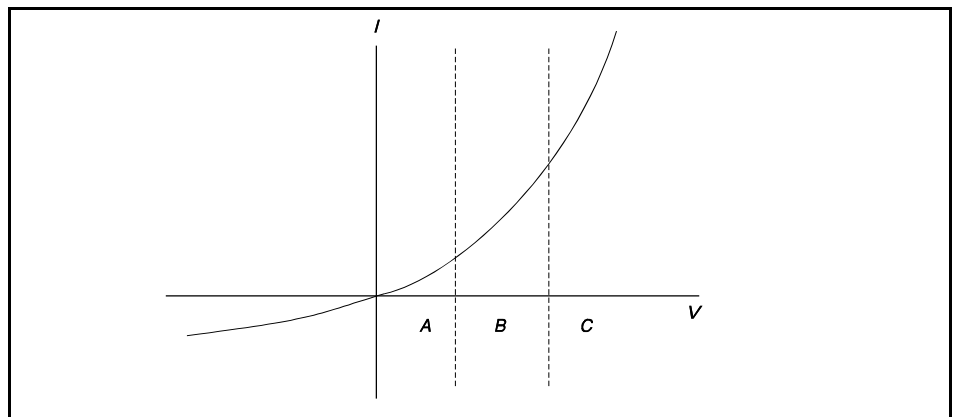
Figure 6-3. Ideal Diode Response
