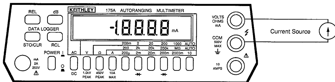
Figure 2-6. Current Measurements up to 2000mA
