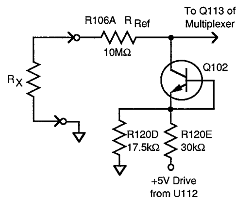
B. 20kΩ and 200kΩ Ranges
