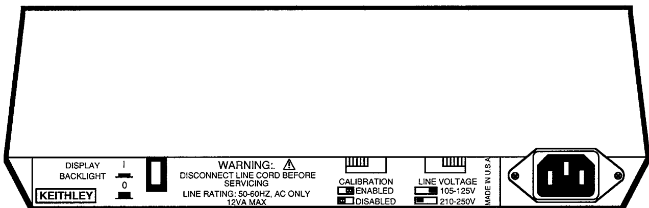
Figure 5-3. Model 175A Rear Panel
