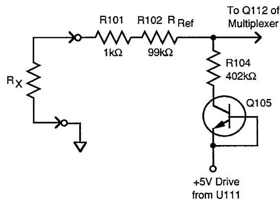
A. 200Ω and 2kΩ Ranges
