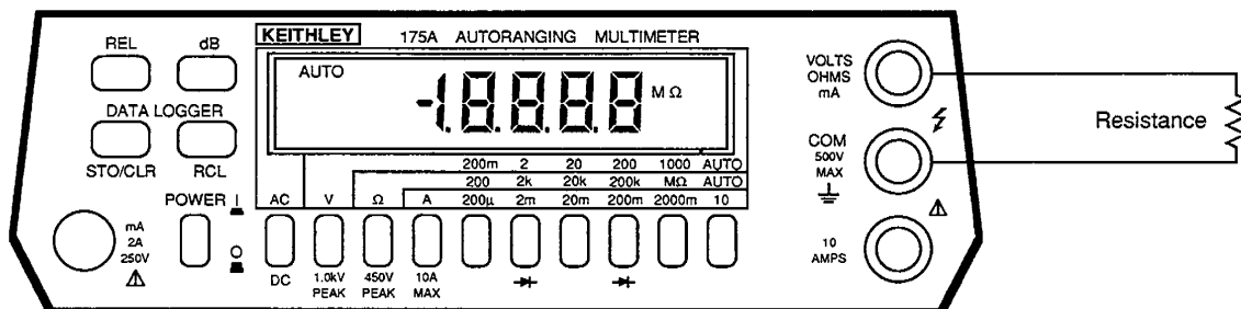
Figure 2-4. Resistance Measurements
