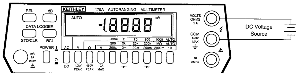
Figure 2-2. DC Voltage Measurements
