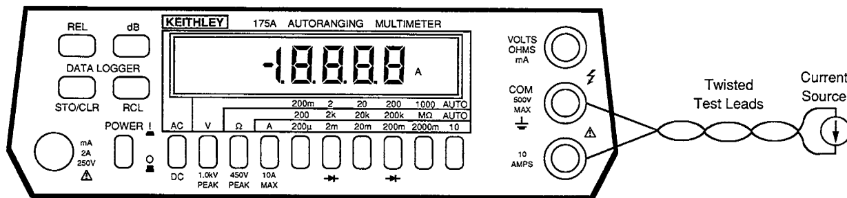
Figure 2-5. Current Measurements between 2000mA and 20A
