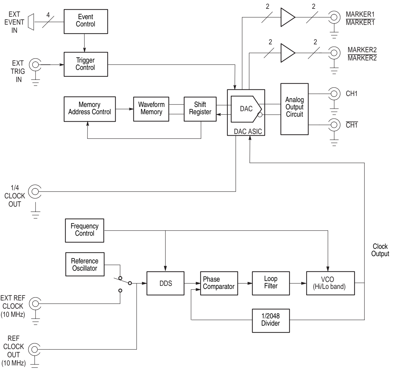
Figure 2-27: AWG710 block diagram
