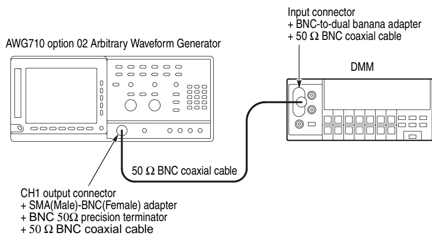
Figure B-46: Option02 output amplitude accuracy initial test hookup
