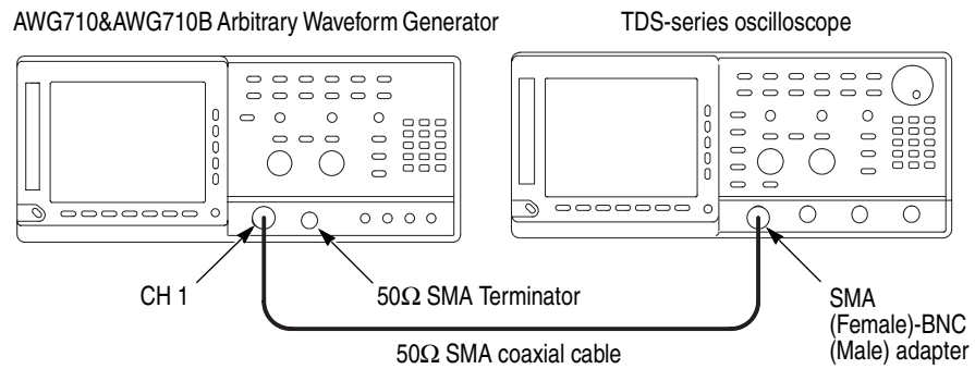
Figure 2-30: Cable connection between AWG710&AWG710B Arbitrary Waveform Generator and digital storage oscilloscope
