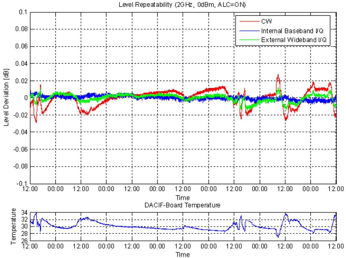
Measured level repeatability over 6 days with random settings between measurements (DACIF board temperature: internal temperature test point, variations caused by changes of ambient temperature).
