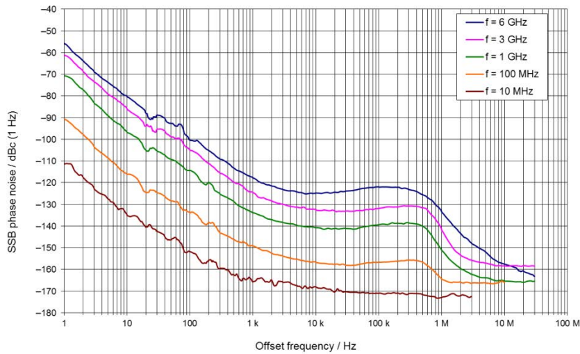
Measured SSB phase noise with internal reference oscillator (with R&S® SMA-B22 enhanced phase noise performance and FM/φM modulator option).
