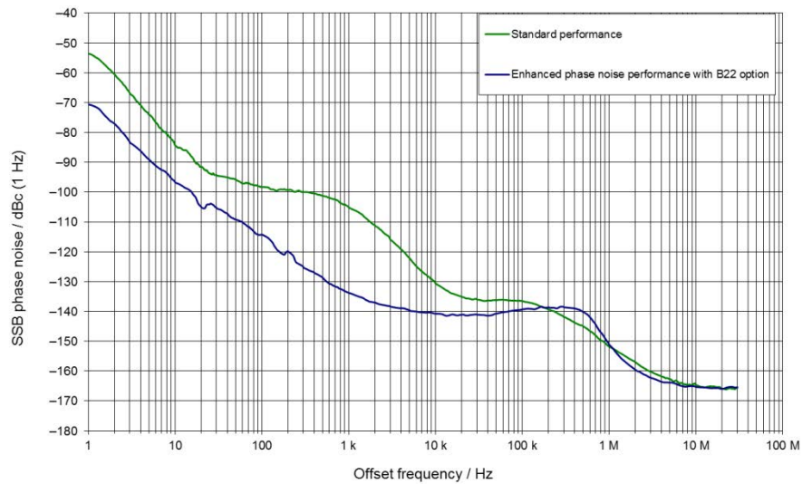
Measured SSB phase noise, f = 1 GHz, comparison of standard performance and performance with R&S®SMA-B22 option.
