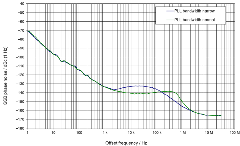
Measured SSB phase noise, f = 1 GHz (with R&S® SMA-B22 enhanced phase noise performance and FM/φM modulator option), comparison of PLL bandwidth normal and narrow (only available for f \leq 3 GHz).
