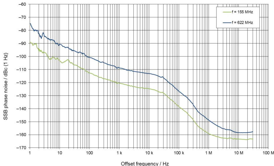
Clock synthesizer (R&S®SMA-B29 option): SSB phase noise measured with R&S®SMA-B22 option.
