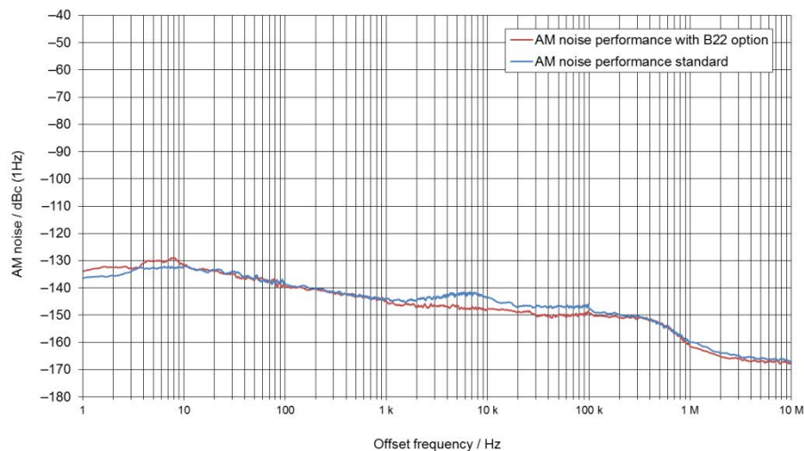
Measured AM noise, f = 1 GHz, level = +14 dBm, ALC ON, comparison of standard performance and performance with R&S®SMA-B22 option.
