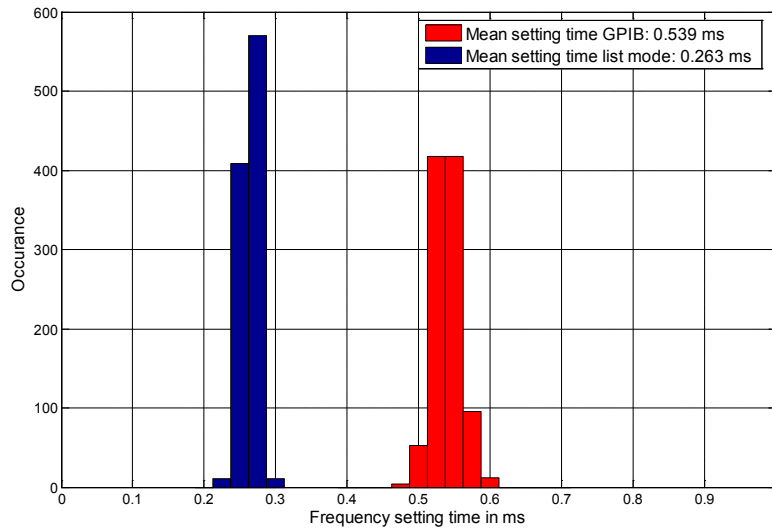
Histogram over 1000 frequency setting time measurements with GPIB remote control and List mode.
