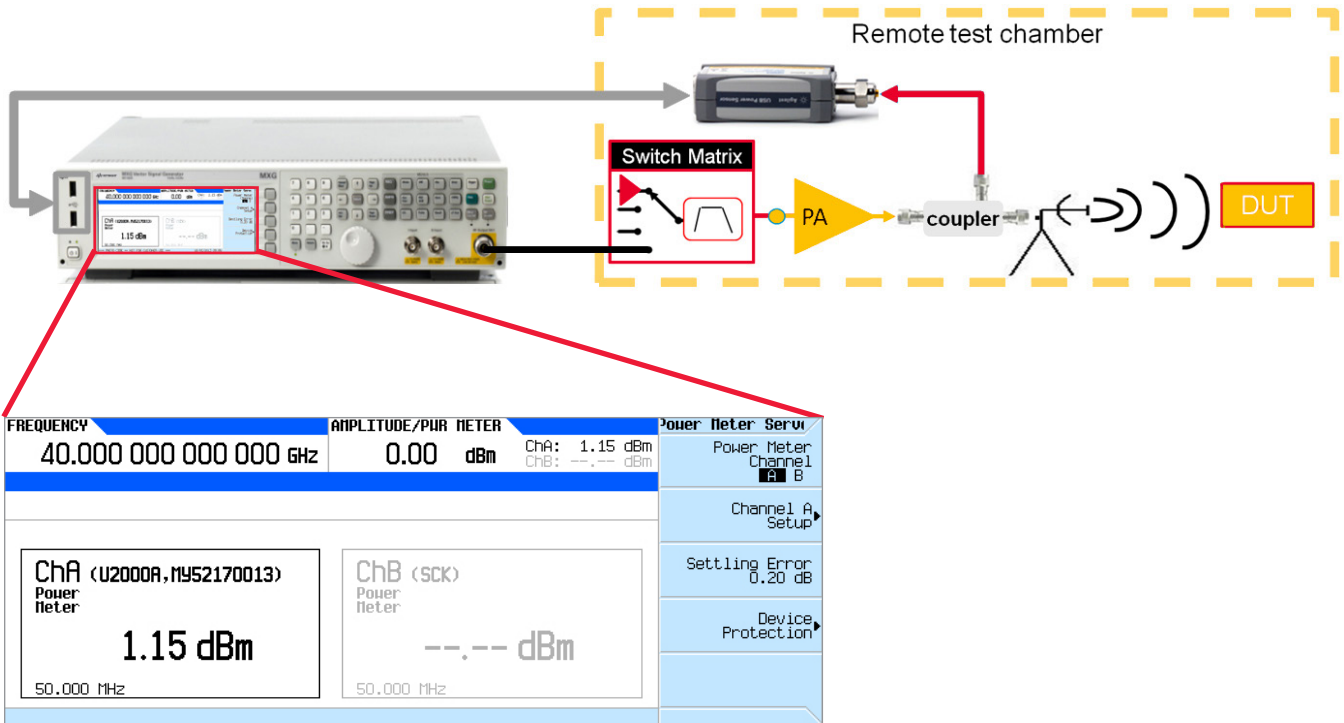
Use automatic leveling on the MXG or EXG to calibrate your device
