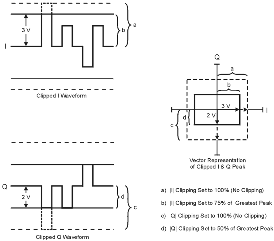
Figure 3-15 Rectangular Clipping
