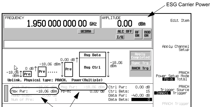
Figure 16-22 Offset Power
