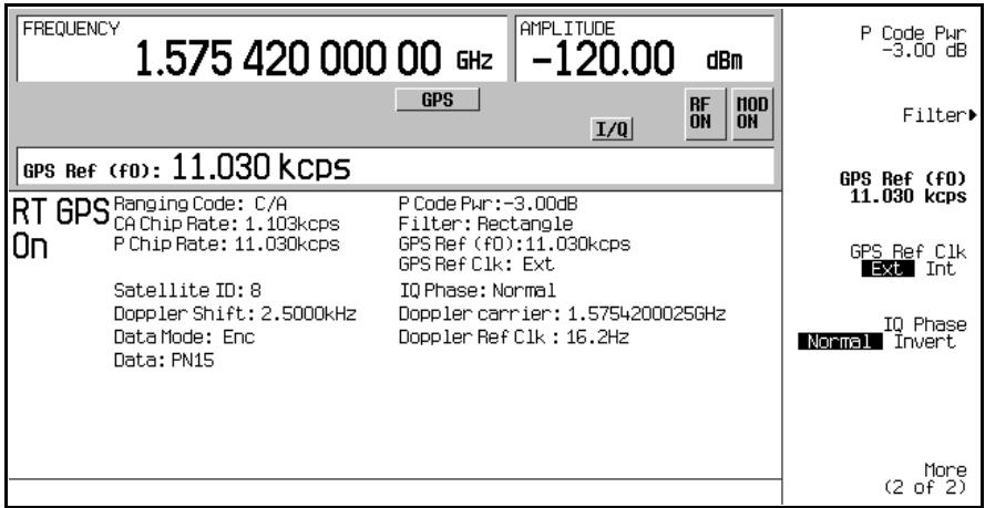
Figure 11-7 Real Time GPS Setup with External Clock
