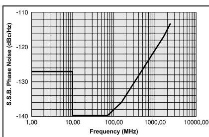
Typical Phase Noise at 20 kHz offset
