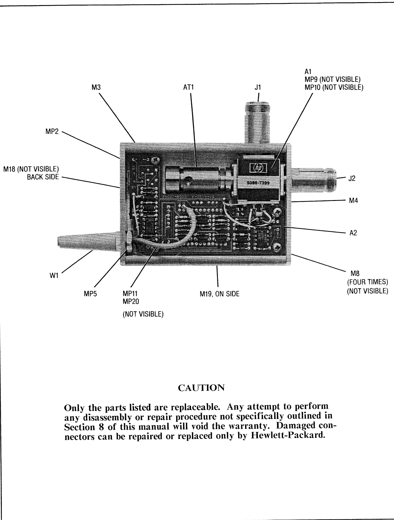
Figure 6-1C. HP 85027C Replaceable Parts Identification
