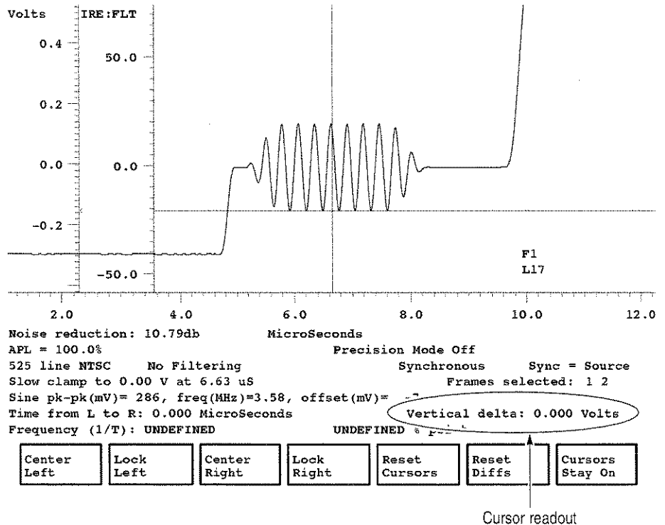
Figure 3-4: Color burst aligned with horizontal reference line
