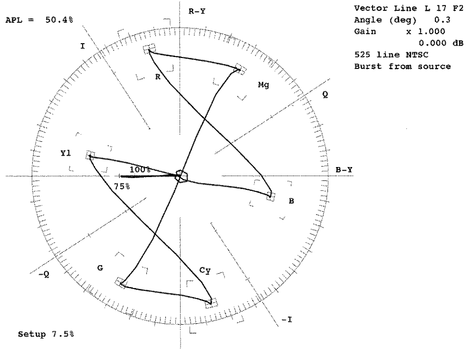
Figure 3-6: Vector display of a color bar signal
