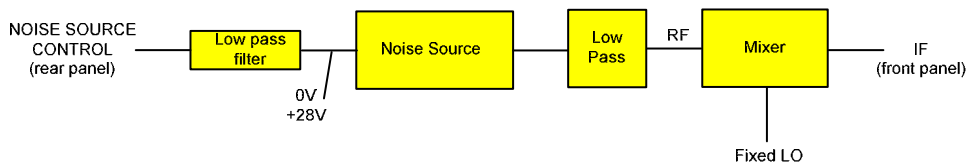
Fig. 2-33: Test setup for the main measurement
