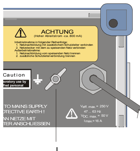
Threaded bolt with butterfly nut on the rear of the device
