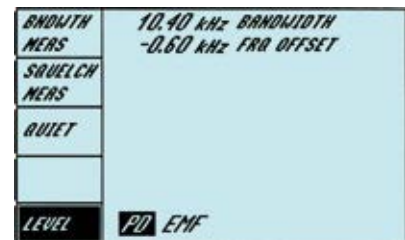
Semi-automatic search routines for squelch level, receiver bandwidth, and sensitivity perform elaborate measurements within a few seconds
