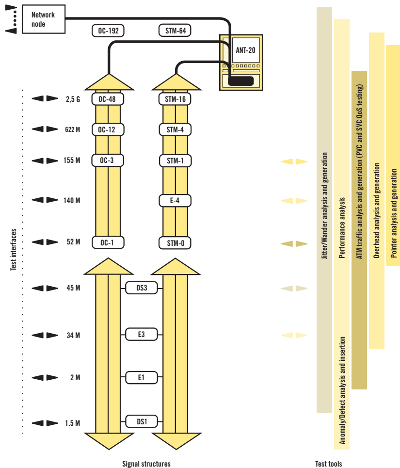
Even at 10 Gbps, ANT-20se can break down signal structures and analyze them down to the lowest levels
