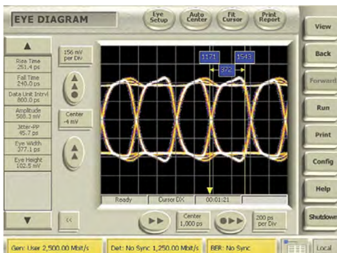
DCD jitter measurement.
