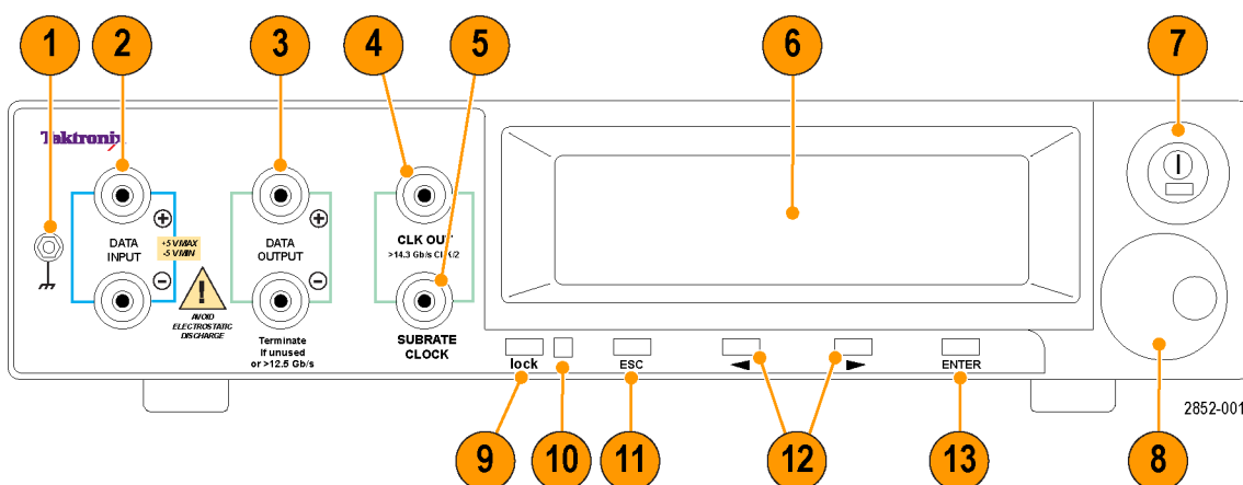
Figure 2: Front panel connectors and controls
