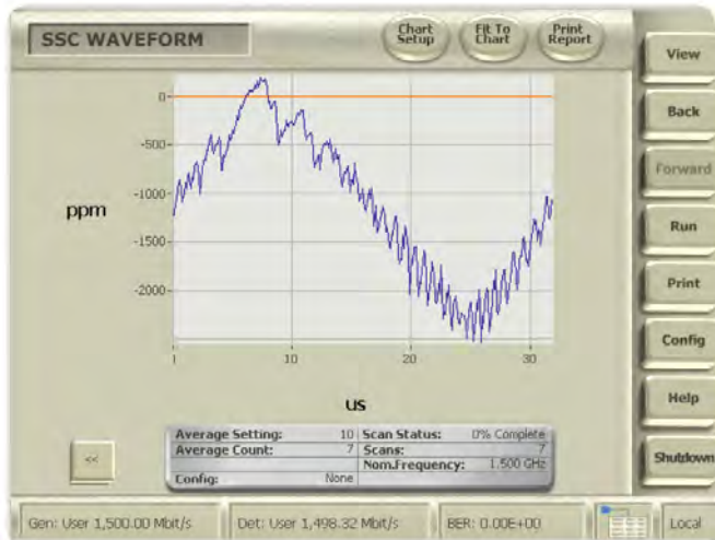
Excessive noise in the SSC modulator may cause tracking problems in the receiver CDR, resulting in bit errors.
