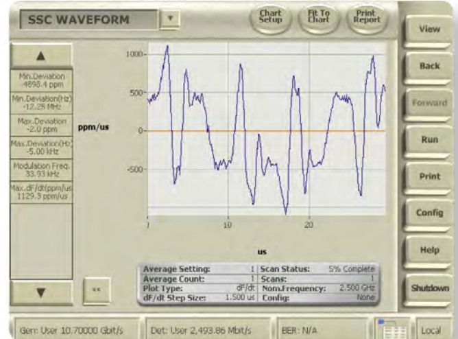
A revealing dF/dT waveform showing poor performance.
