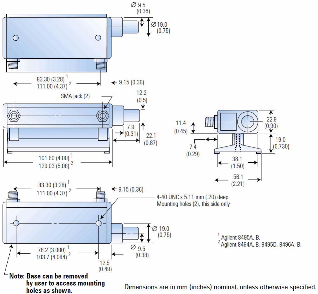
Figure 4 Dimensions of Agilent 8495D Attenuator
