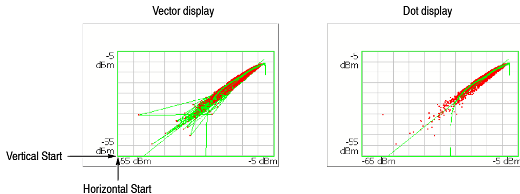
Figure 3-138: Vector and dot displays for AM/AM view
