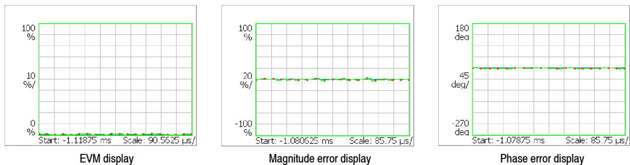
Figure 3- 134: EVM, magnitude and phase error displays
