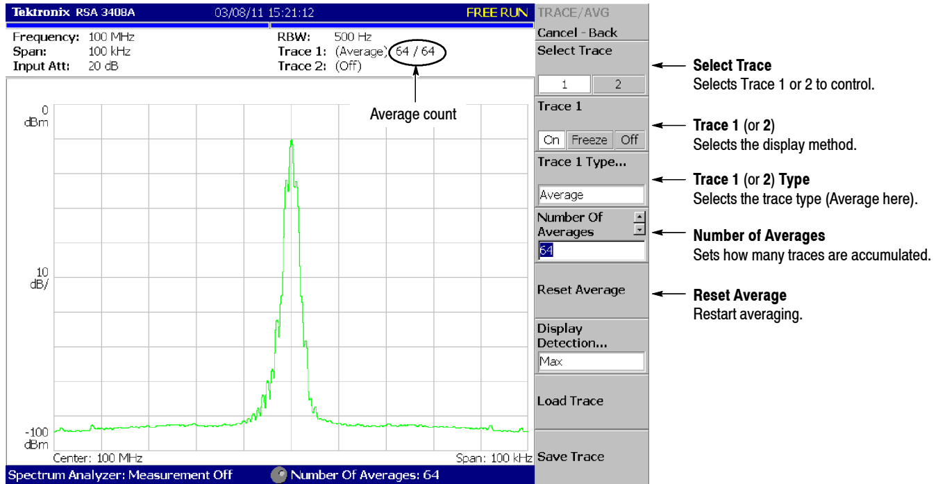
Figure 3- 123: Displaying an averaged waveform
