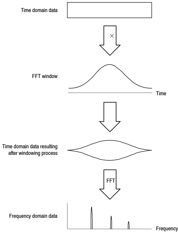
Figure 3-120: Windowing process of time domain data
