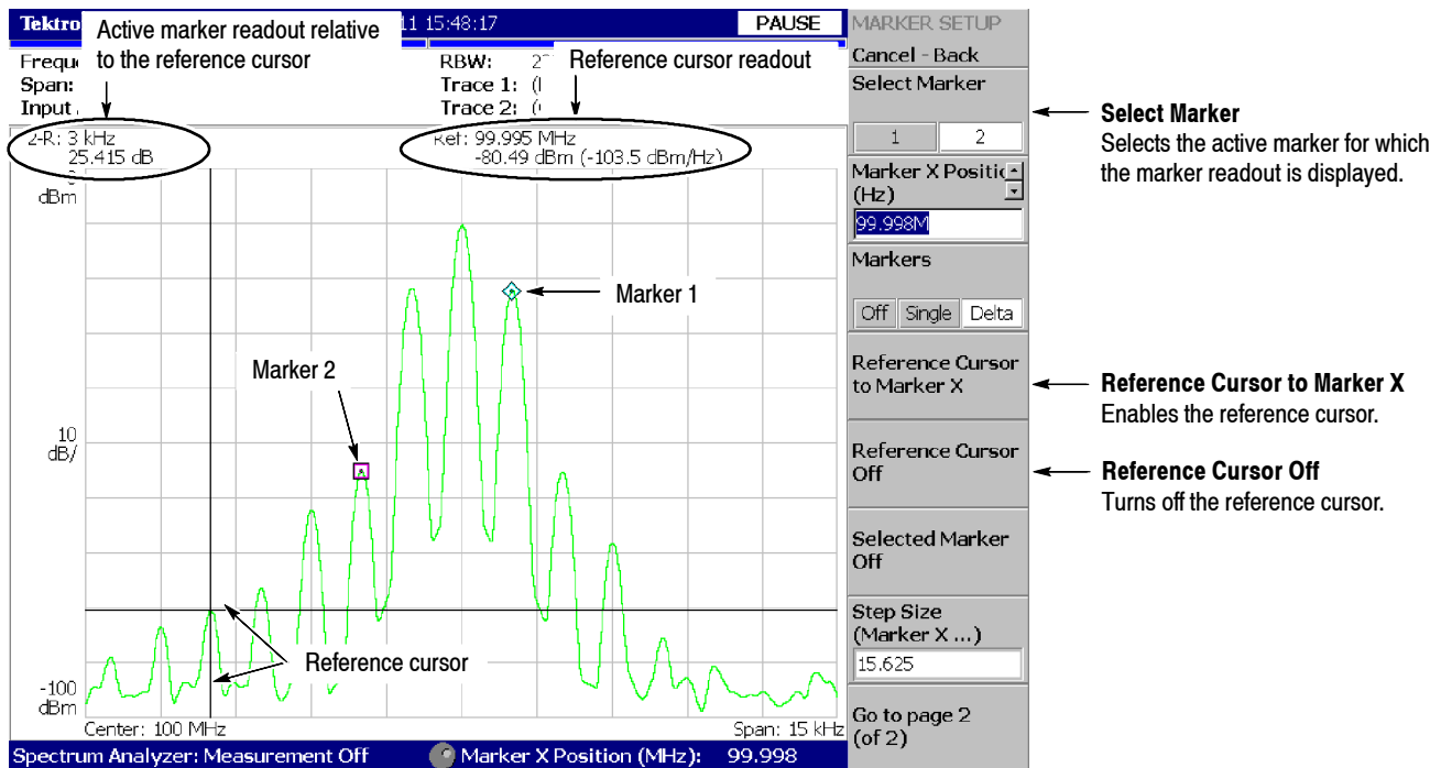
Figure 3-152: Measurement with the reference cursor
