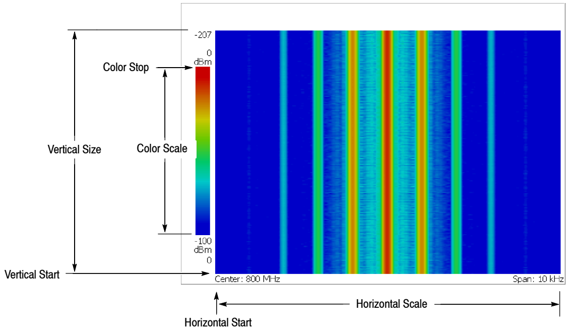
Figure 3- 129: Scale and format settings in spectrogram view
