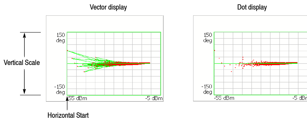
Figure 3-139: Vector and dot displays for AM/PM view
