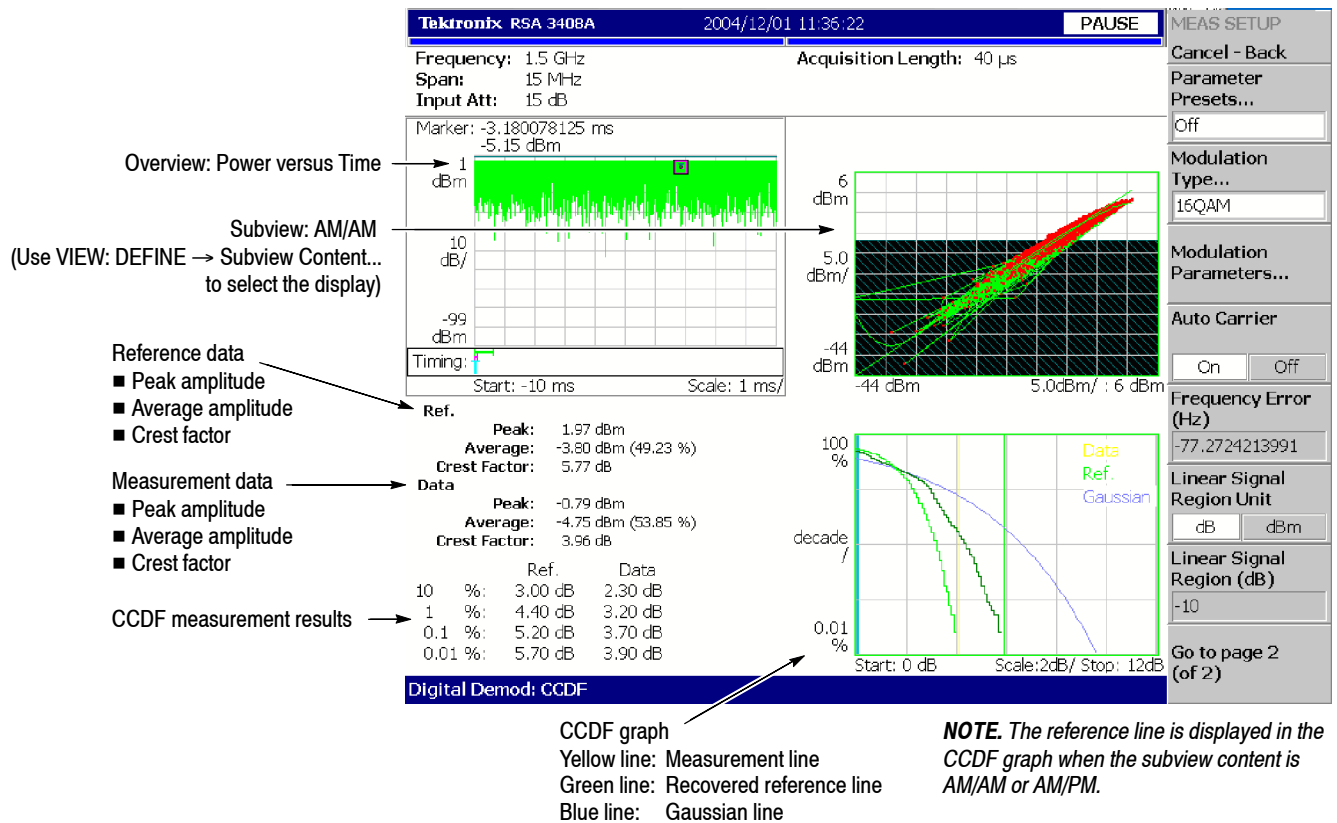
Figure 3-49: CCDF measurement
