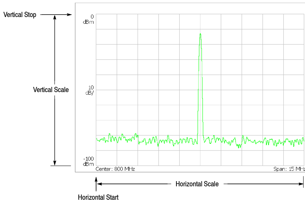
Figure 3- 128: Setting the scale in spectrum view
