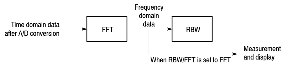
Figure 3-117: Process flow when RBW/FFT = FFT
