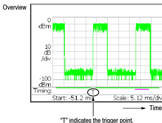
Figure 3-113: Trigger point display
