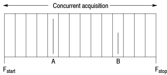
Figure 1-4: Concurrent acquisition
