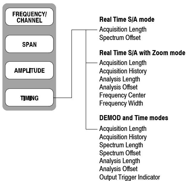
Figure 3-96: Timing menu structure
