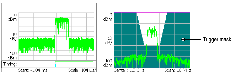
Figure 3-106: Trigger mask
