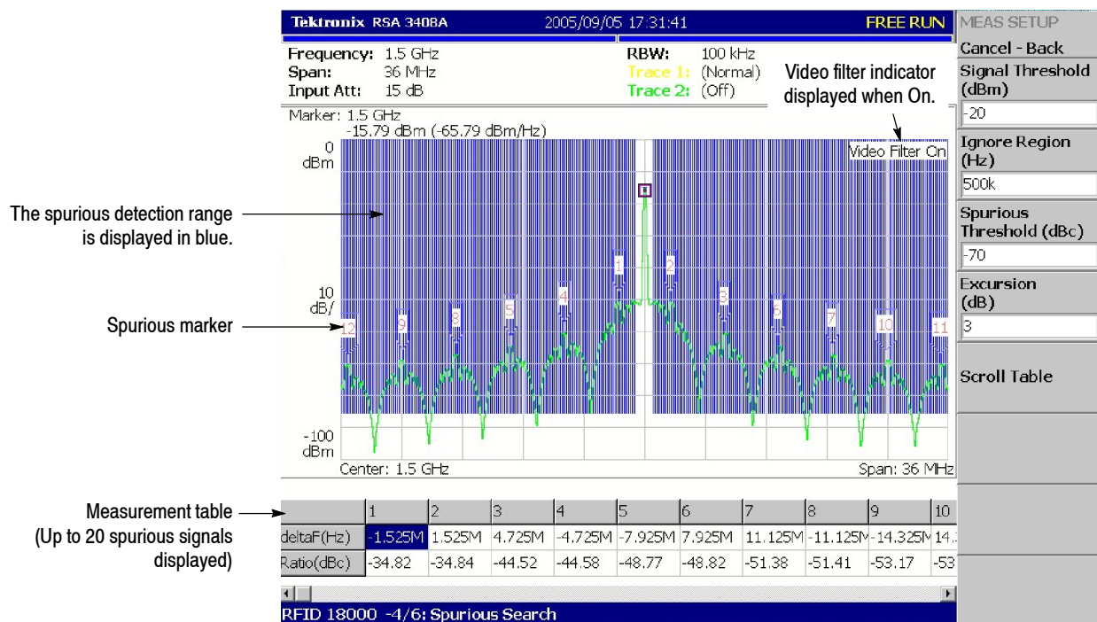
Figure 3-53: Spurious measurement
