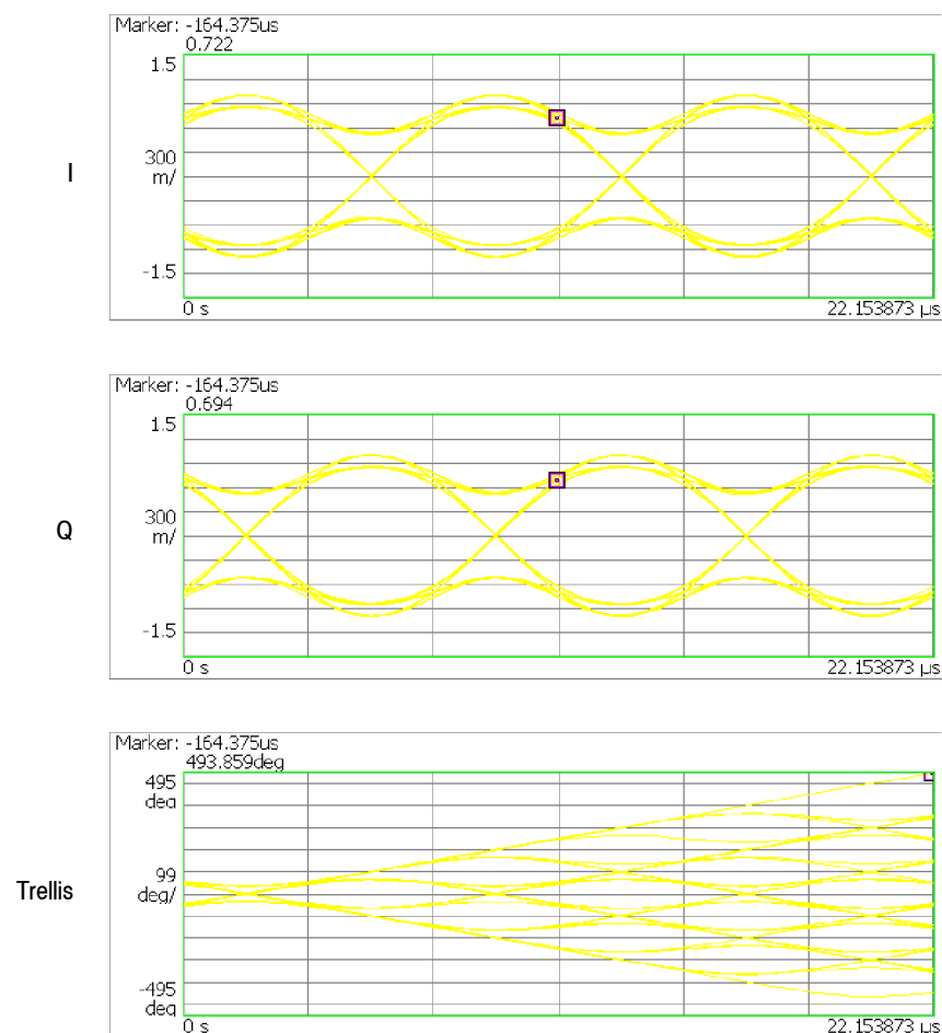
Figure 3-137: Eye diagram view
