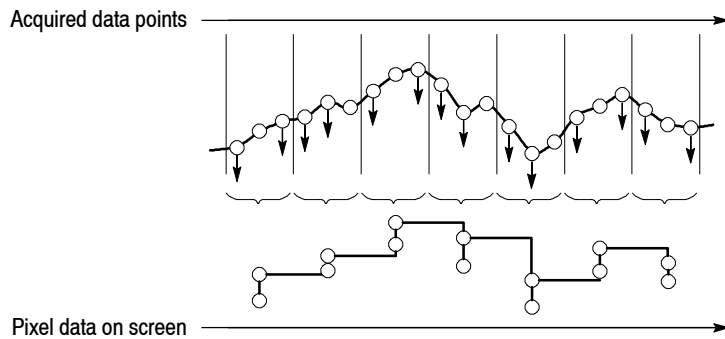
Figure 3- 126: Compression method for displaying the waveform
