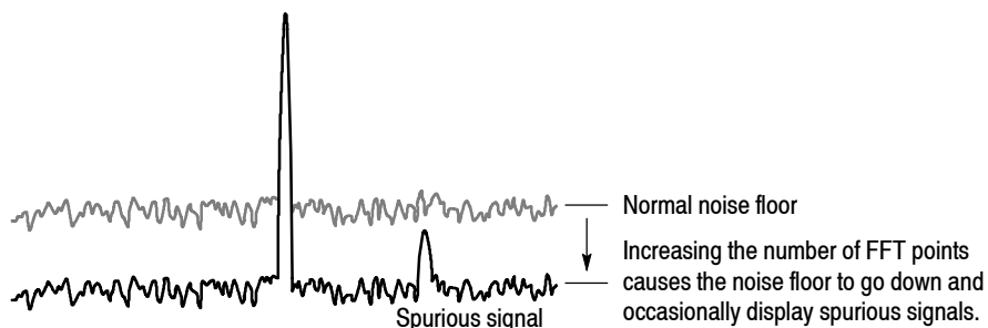
Figure 3-119: Generating spurious signals by increasing the number of FFT points
