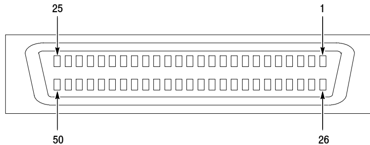
Figure C-1: Digital IQ output connector pin assignment
