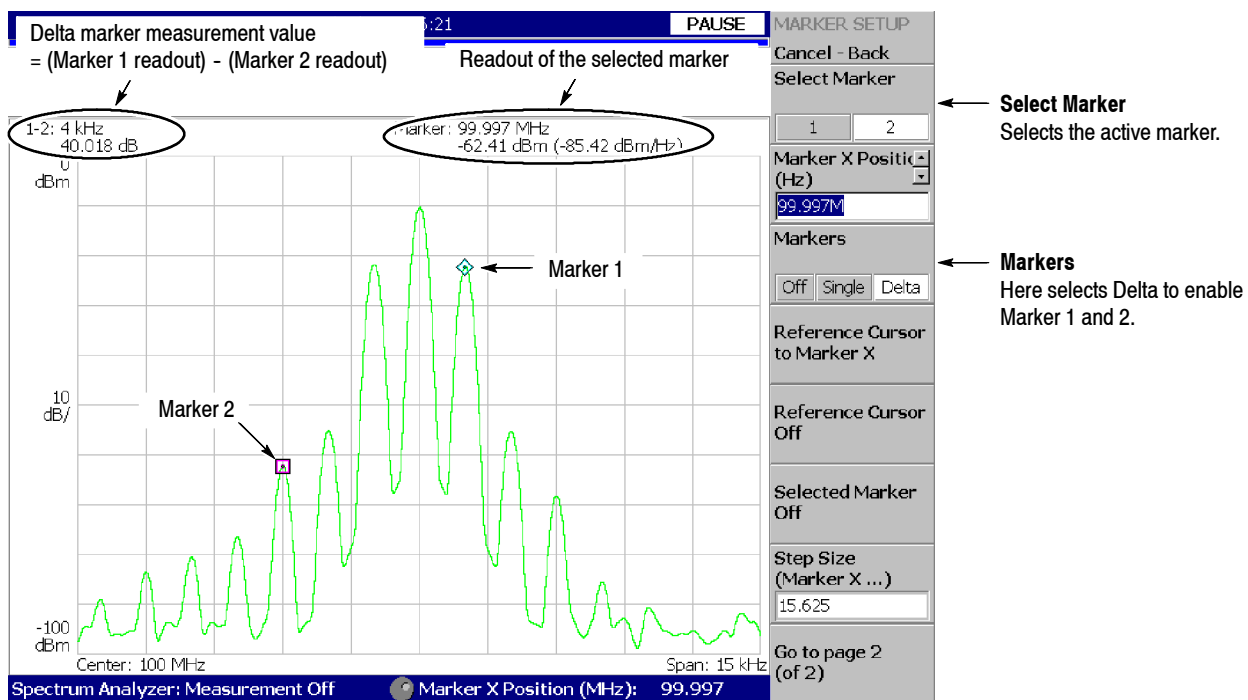
Figure 3- 151: Using the delta marker to take measurements
