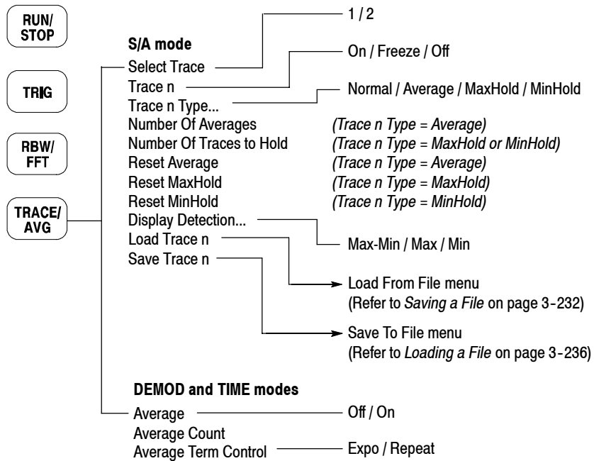
Figure 3- 122: RBW/FFT menu structure
