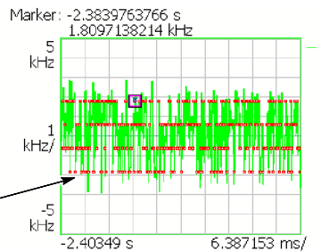
Figure 3-42: IQ/Frequency versus time measurement
