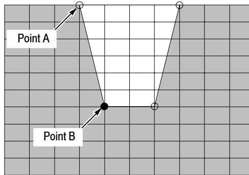
Figure 3- 109: Default mask
