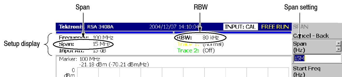
Figure 1-14: Setup display
