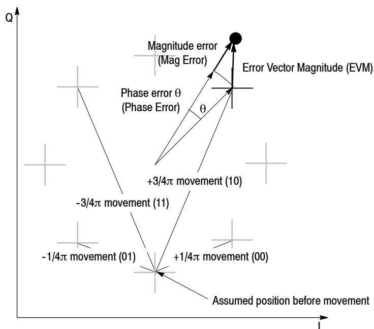
Figure 3-135: Constellation view and error vectors in 1/4\pi QPSK
