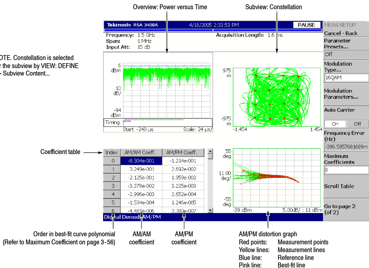
Figure 3-48: AM/PM measurement
