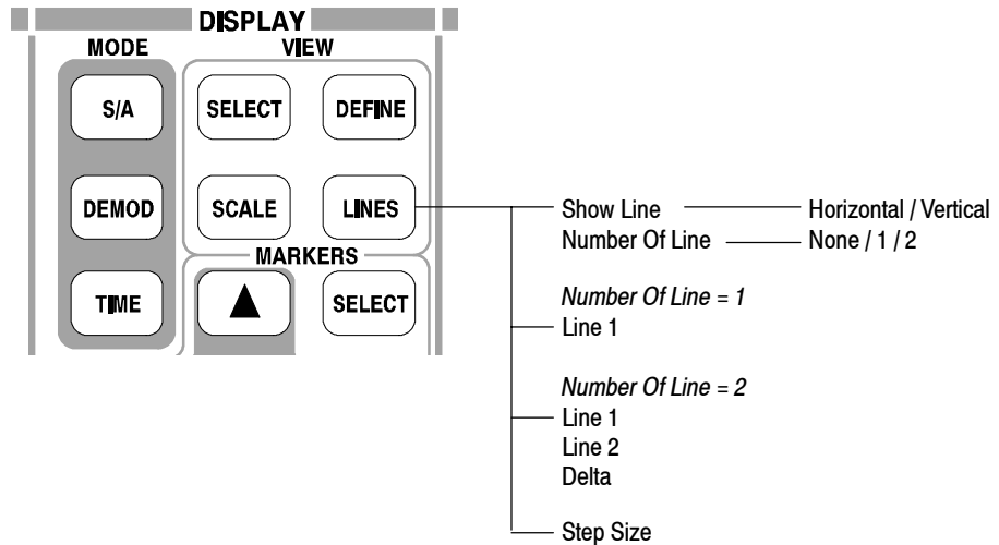
Figure 3- 143: Lines menu structure (other than Real Time S/A)
