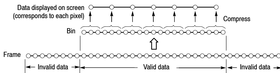
Figure 3-125: Relationships between frame, bin, and pixel
