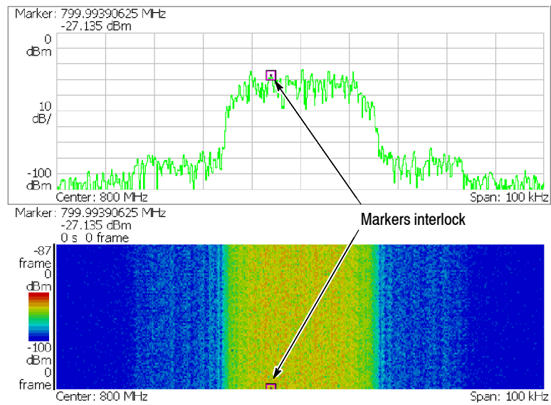
Figure 3-154: Interlocked markers
