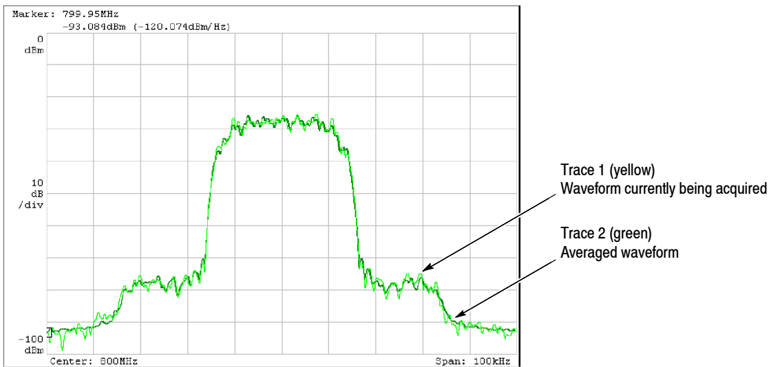
Figure 3-121: Comparison display of Trace 1 and 2
