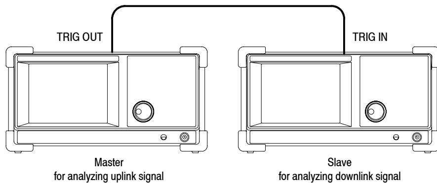
Figure 3- 114: Synchronous operation of two RSA3408A analyzers
