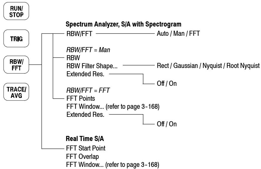
Figure 3- 116: RBW/FFT menu tree
