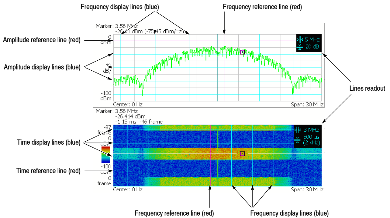
Figure 3-146: Multi display lines (Real Time S/A mode)
