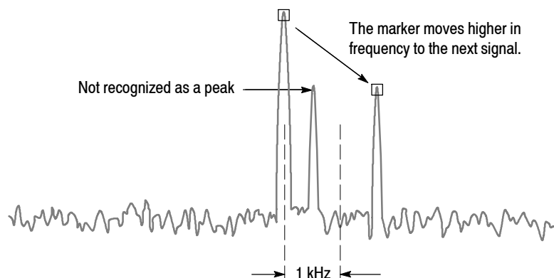
Figure 3-156: Setting the minimum frequency jump
