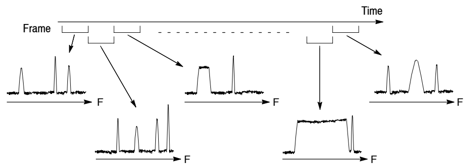
Figure 1-5: Frame acquisition
