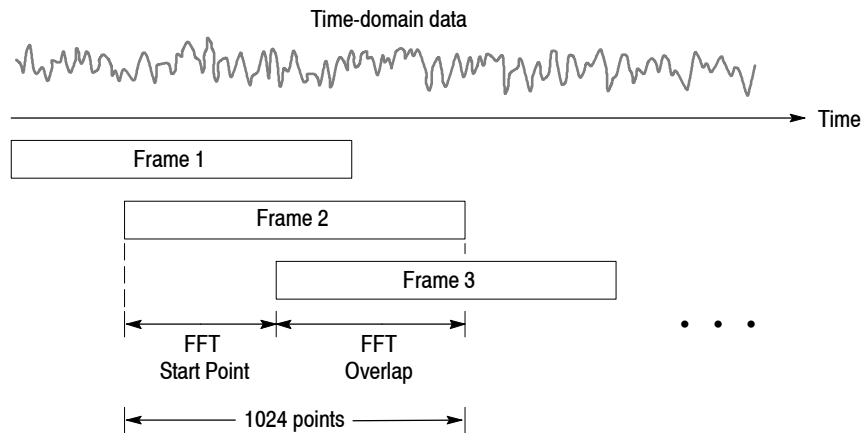
Figure 3- 118: FFT overlap
