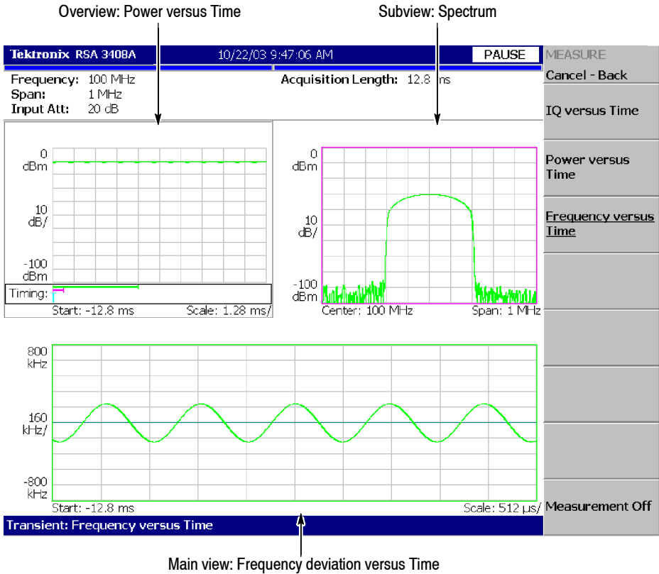
Figure 3-65: Frequency measurement
