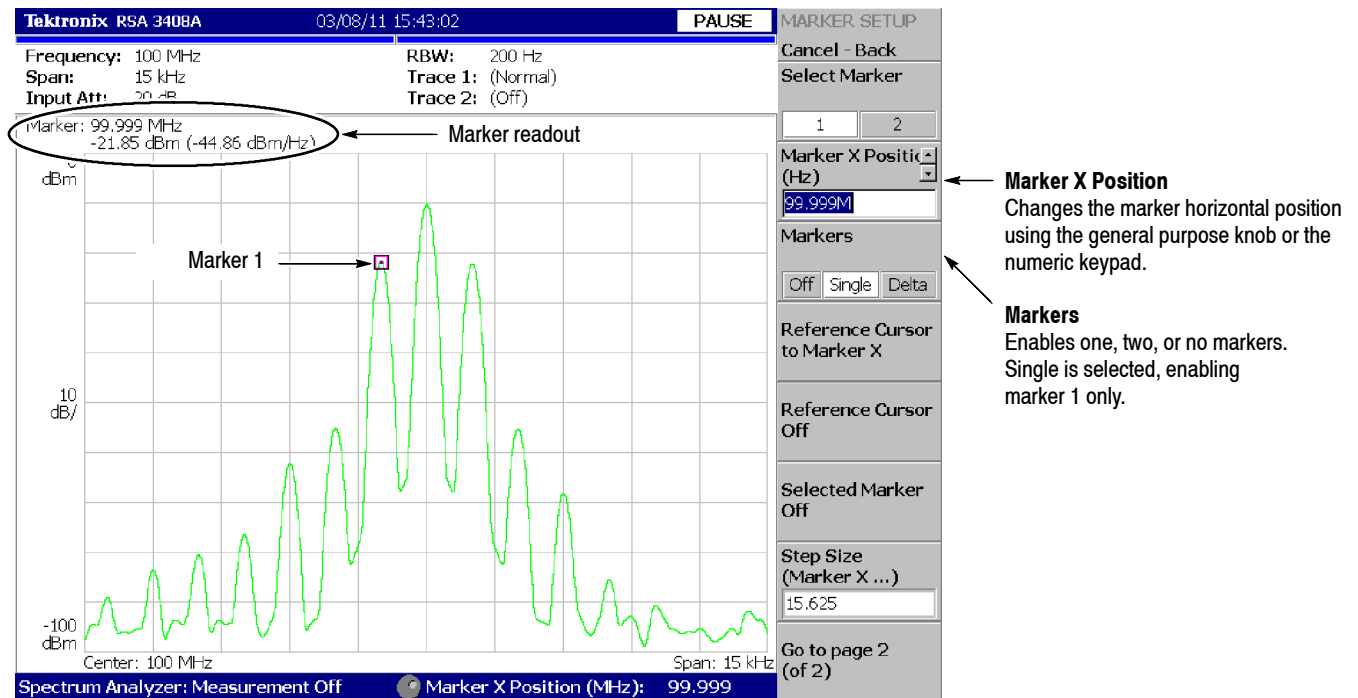
Figure 3-150: Measurement with a single marker
