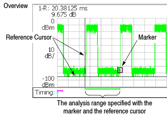
Figure 3-29: Specifying the range with the marker and the reference cursor
