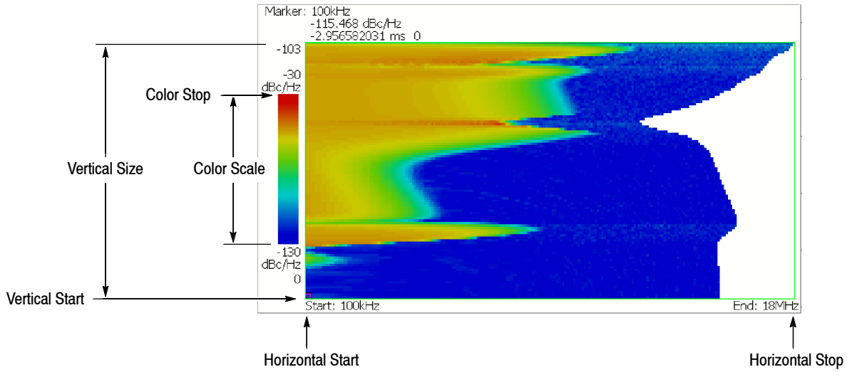
Figure 3- 141: Setting the scale in noisogram view
