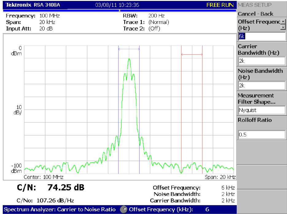
Figure 3-9: Example of C/N measurement
