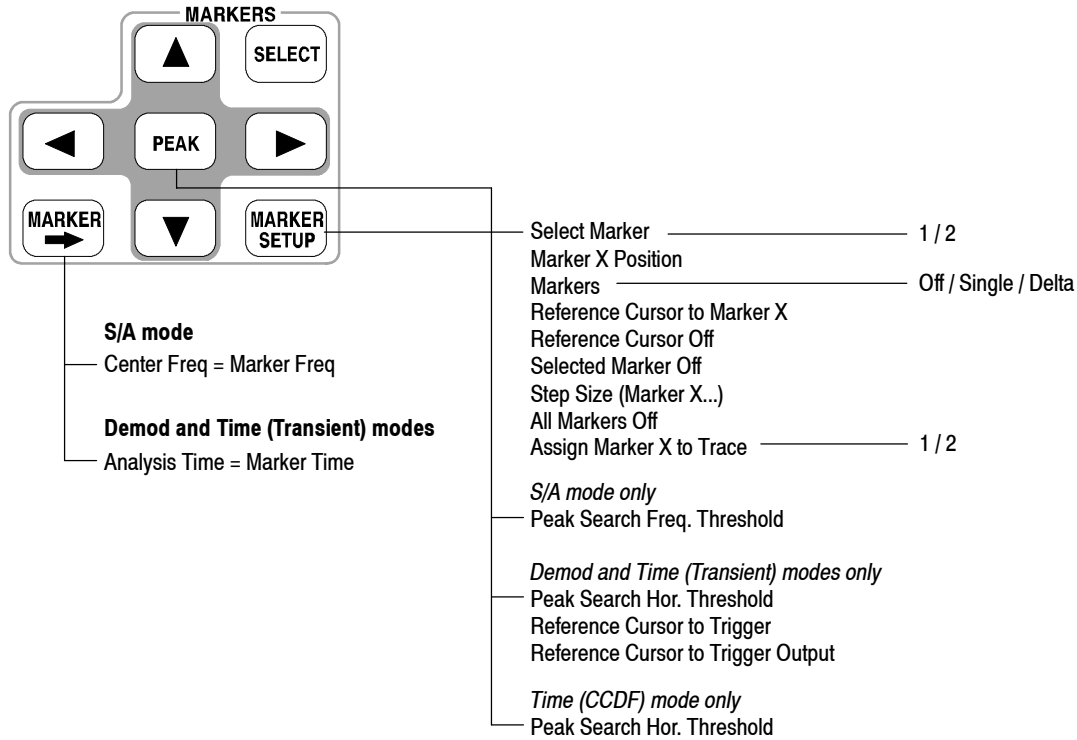
Figure 3- 149: Markers menu structure
