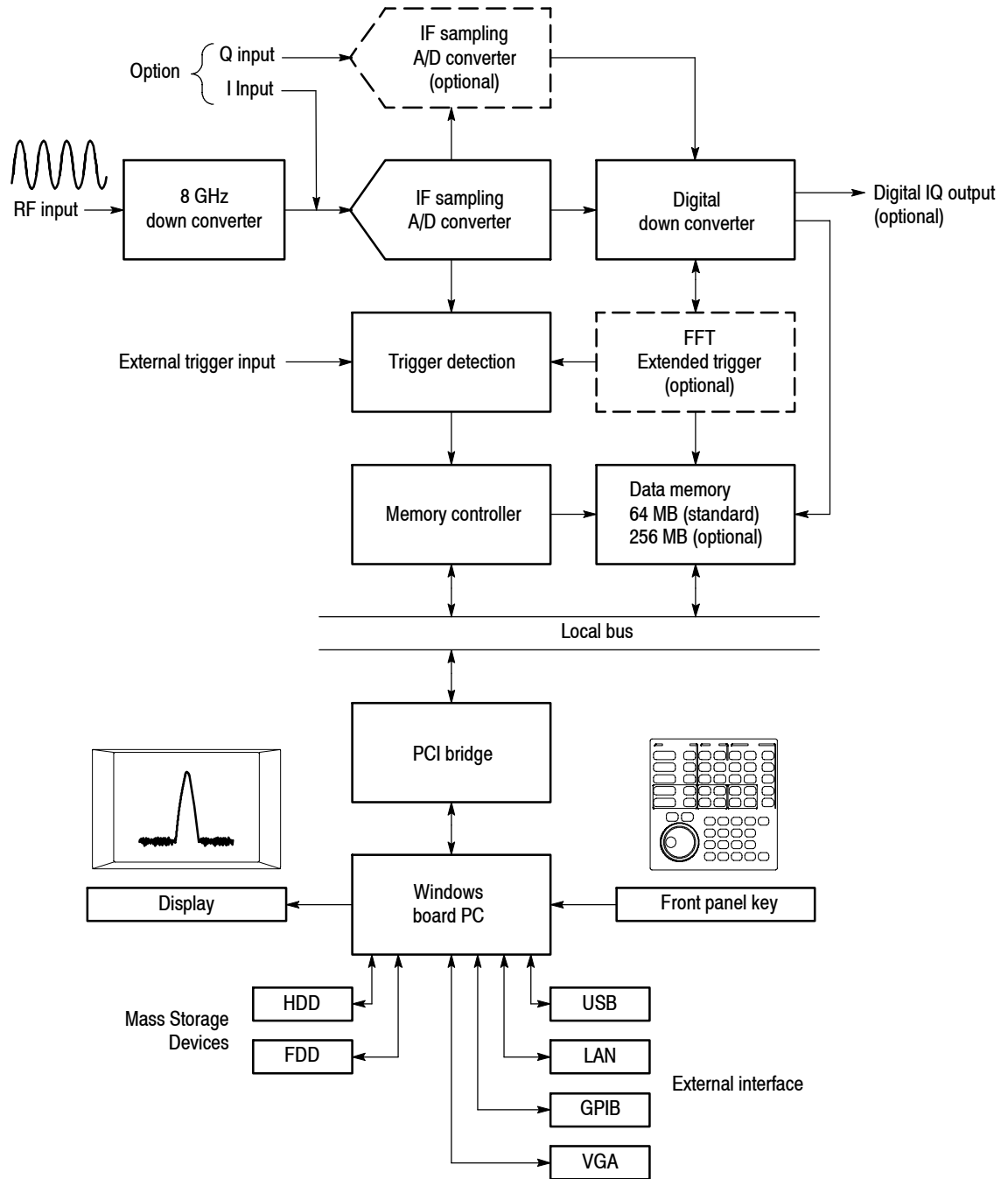
Figure 1-6: Block diagram
