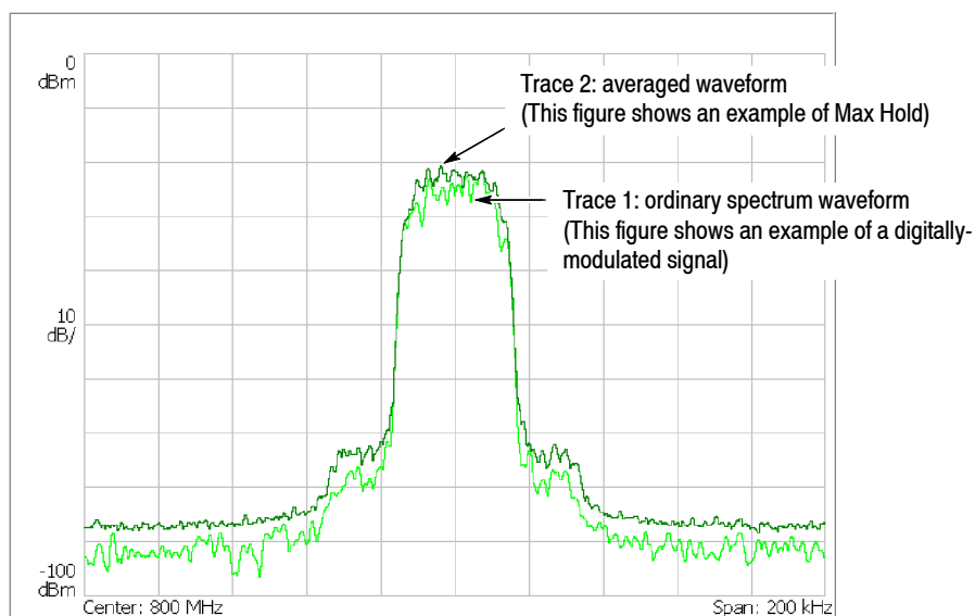
Figure 3-124: Compared display
