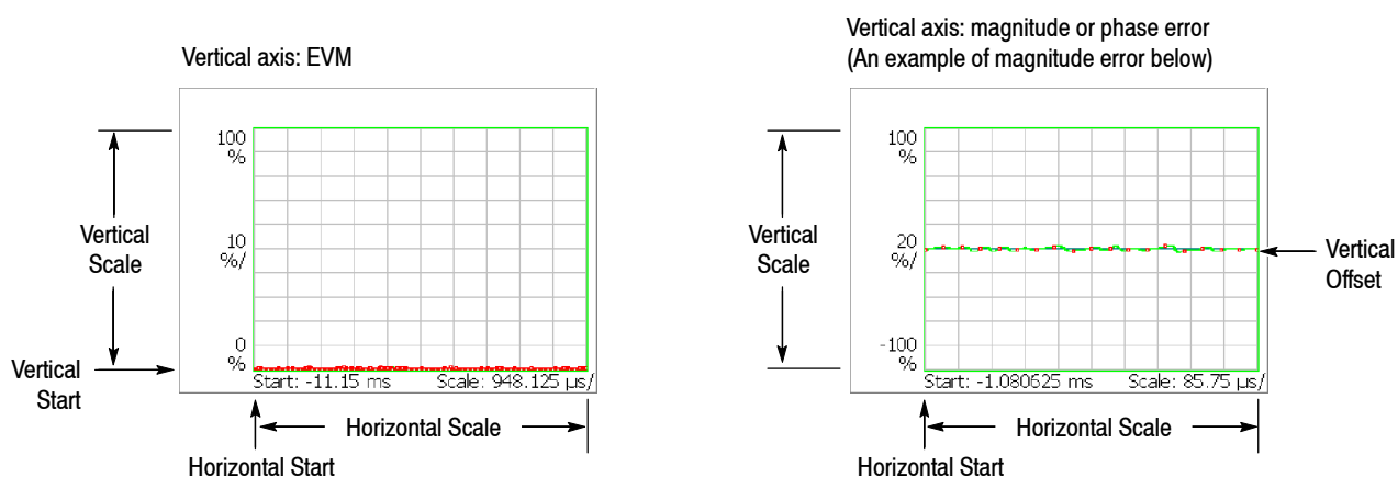
Figure 3-133: Setting the scale in EVM view
