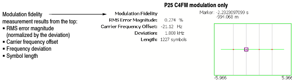
Figure 3-40: Constellation analysis
