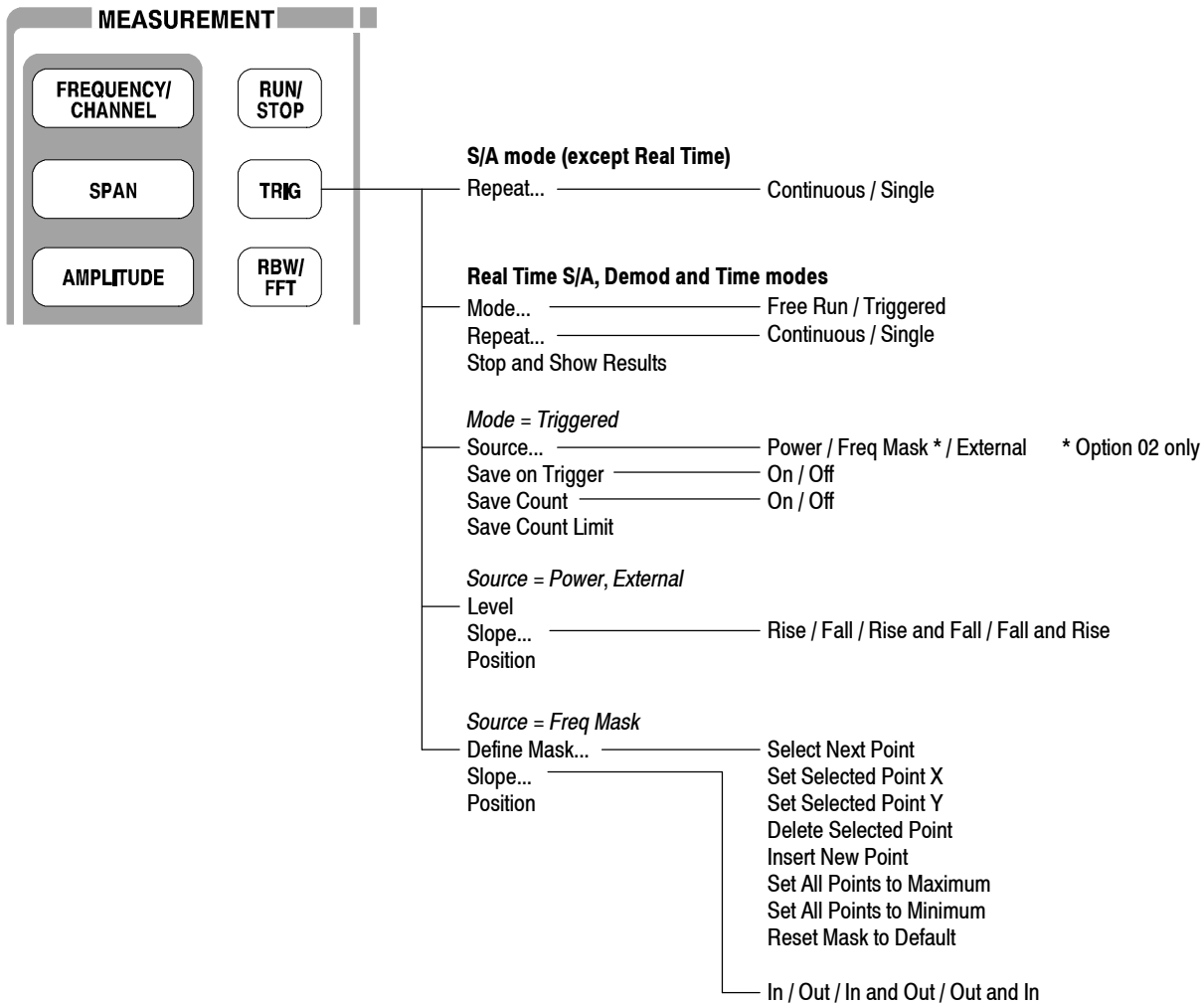
Figure 3- 101: Trigger menu structure
