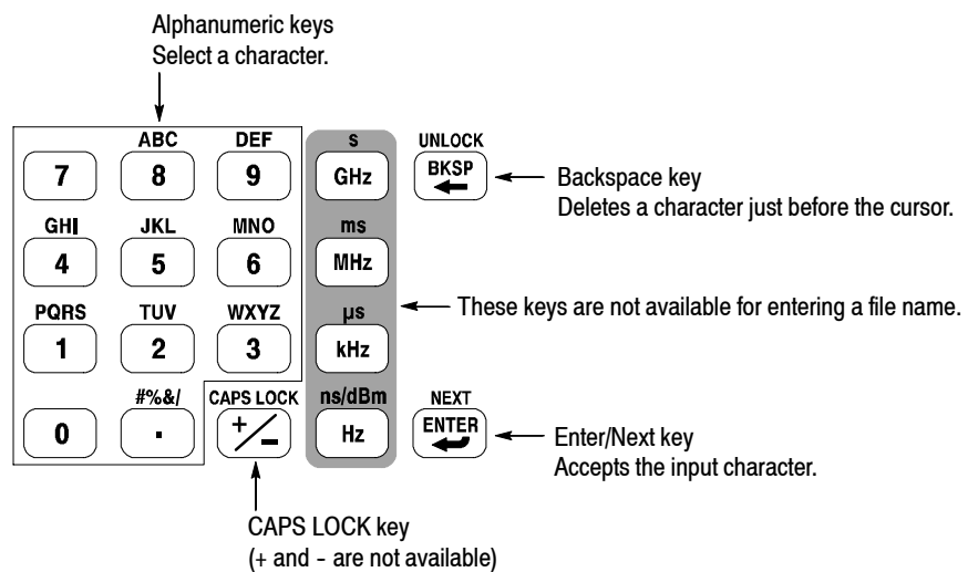
Figure 3- 167: Alphanumeric keypad
