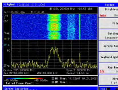
The N9340B INM shows spectrogram and spectrum trace on the same screen.
