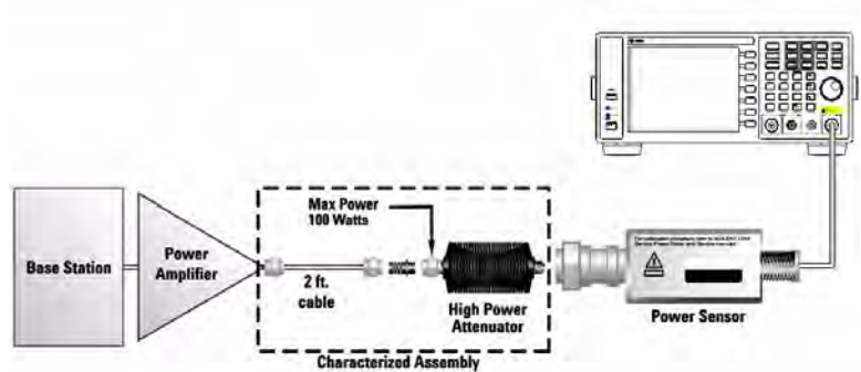
Figure 3-25 Connection with base station
