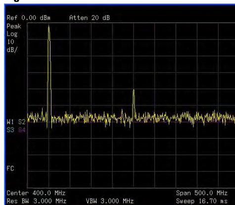
Figure 3-16 Harmonic Distortion
