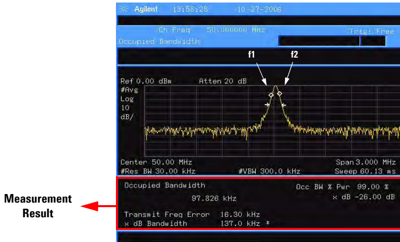
Figure 4-5 Occupied Bandwidth Measurement
