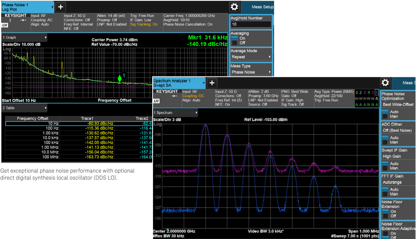
Accurately measure low-level signals to reduce measurement noise by up to 10 dB with Noise Floor Extension (NFE).
