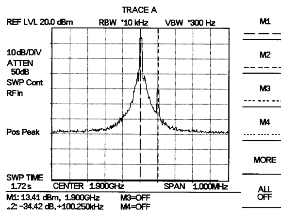
Figure 4-3. Measurement of Two Signals Having Unequal Amplitudes
