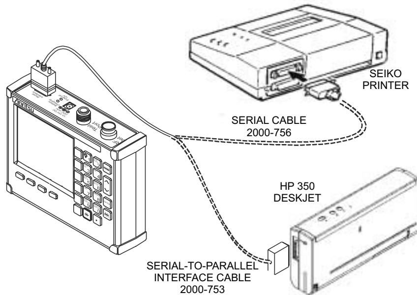
Figure 2-12. Printer Setup
