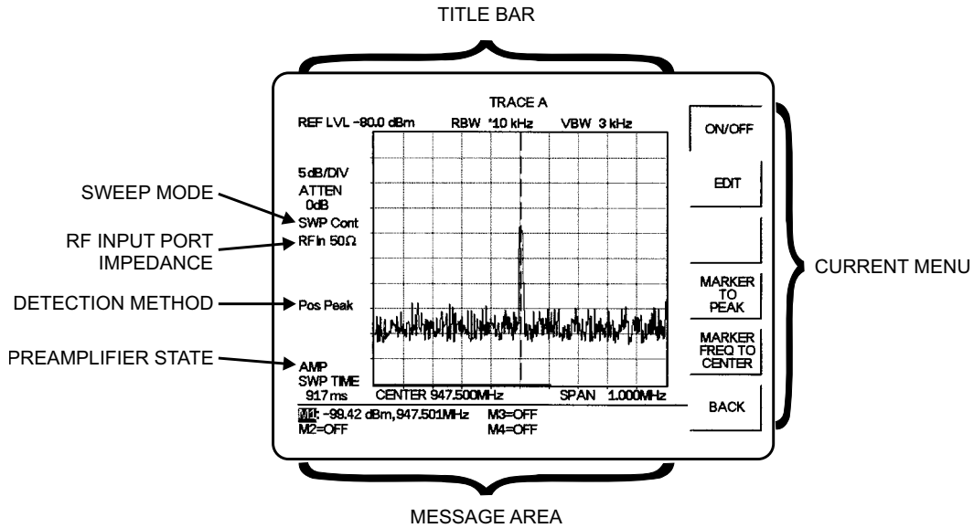
Figure 2-3. Display Overview
