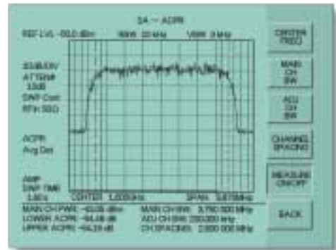
ACP Measurement
