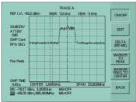
Preamp Off
