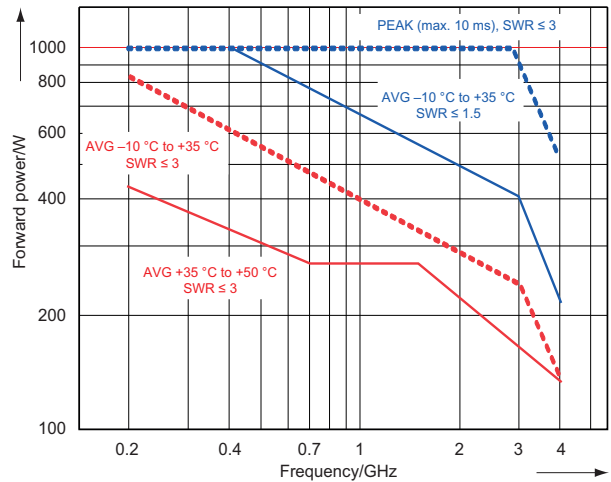
Power-handling capacity.
