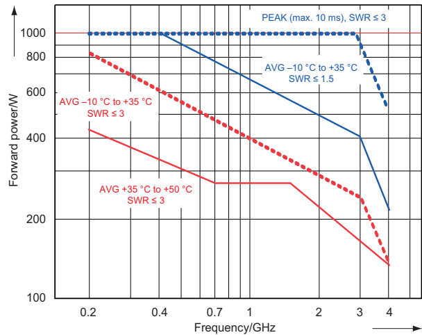
Power-handling capacity.
