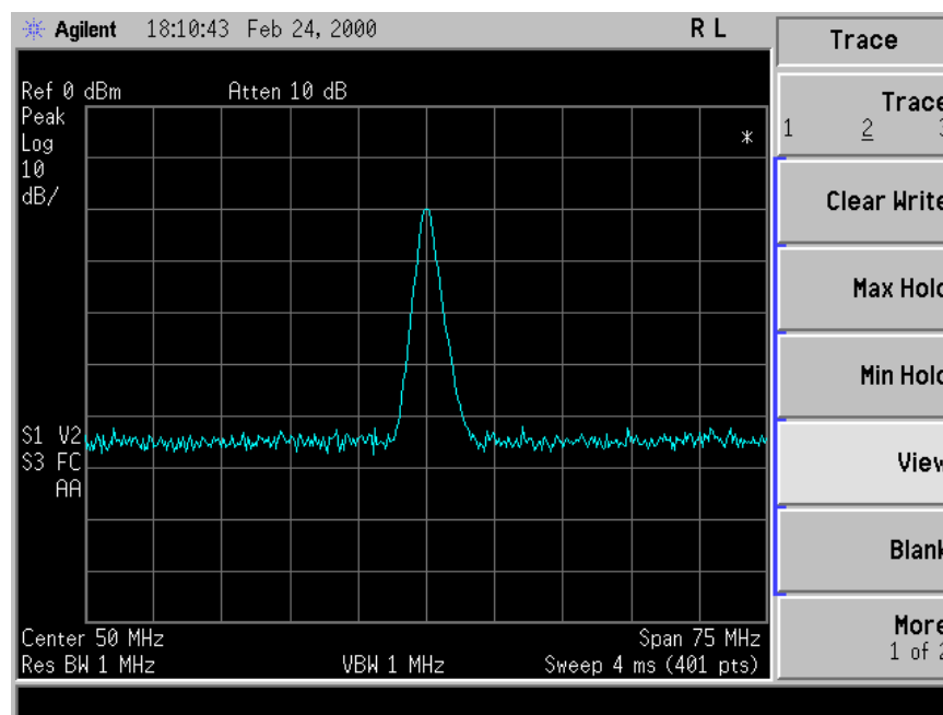
Figure 4-7. Verifying Trace 1
