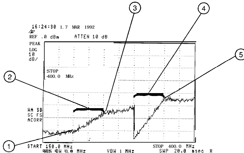
Figure 5-13. Amplitude-Correction Points
