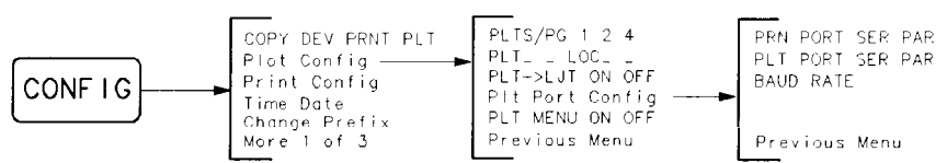
Figure 6-1 1. Baud Rate Menu Map
