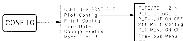
Figure 6-12. Plot Configure Menu
