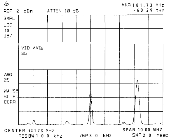
Figure 3-20. Using the Video Averaging Function
