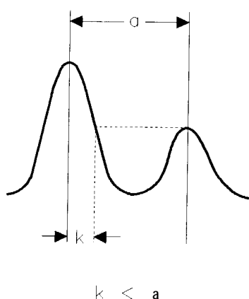
Figure 3-3. Resolution Bandwidth Requirements for Resolving Small Signals
