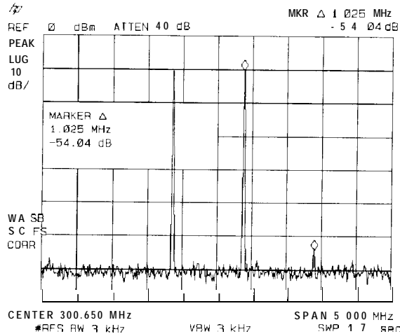
Figure 4-36. Third-Order Intermodulation Measurement
