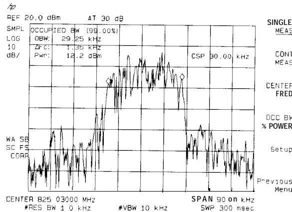
Figure 4-37. Occupied Bandwidth
