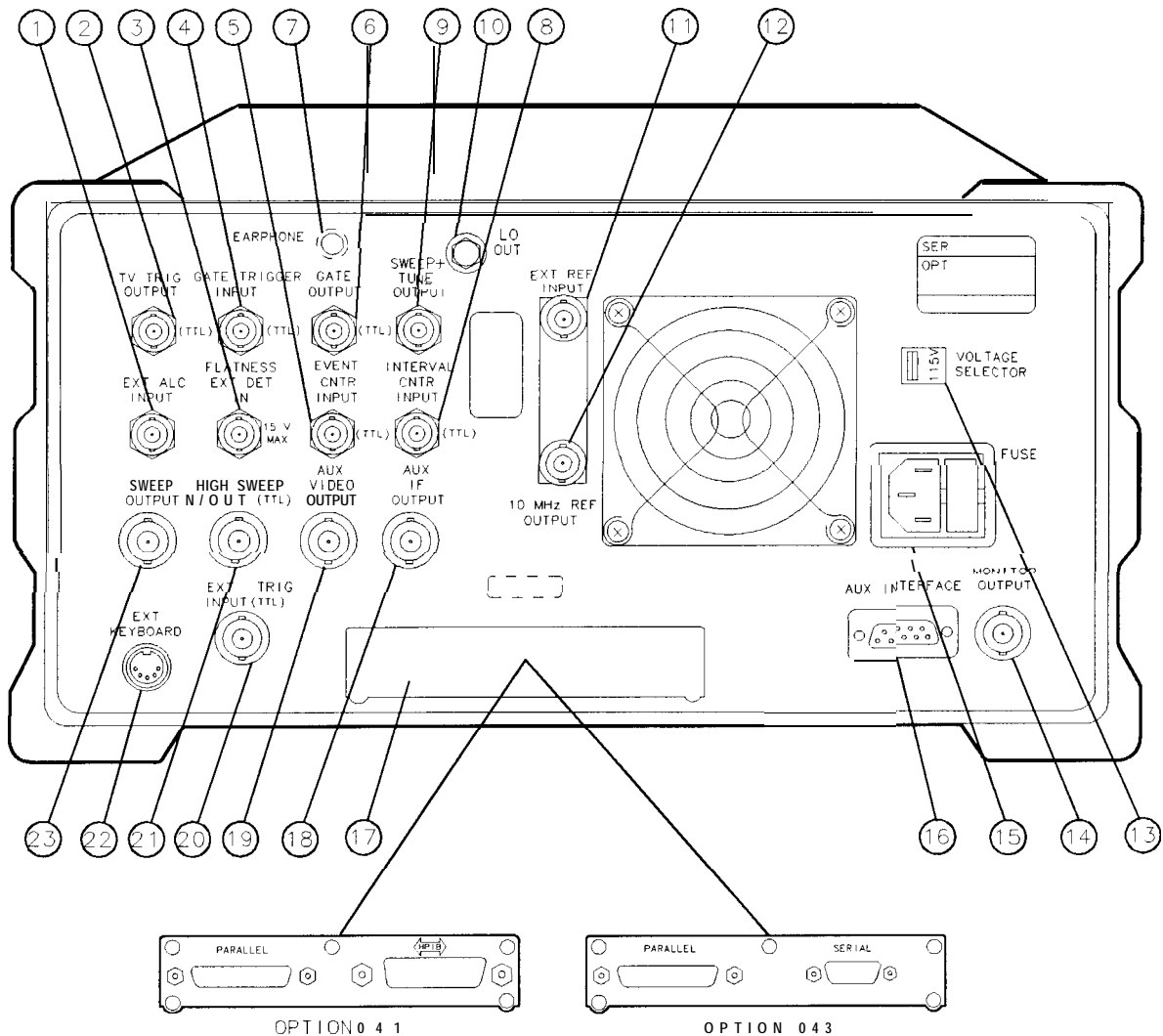
Figure 2-2. Rear-Panel Feature Overview
