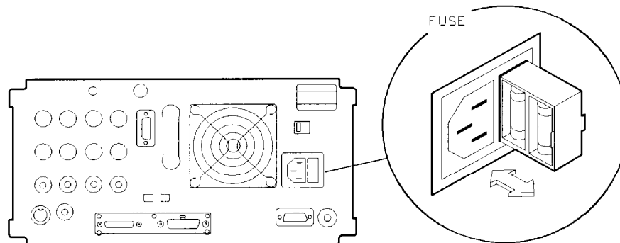
Figure 1-3. Checking the Line Fuse
