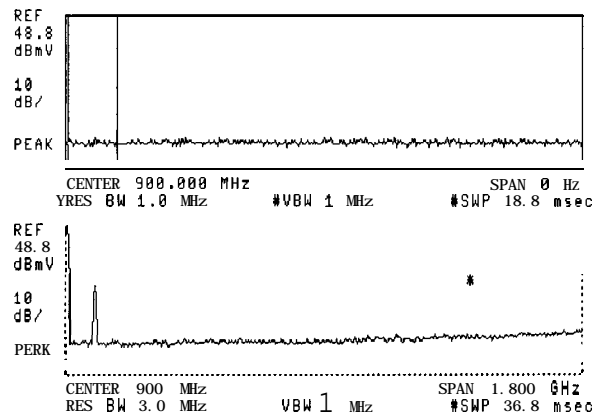
Figure 4-17. Time-Gate Utility Display
