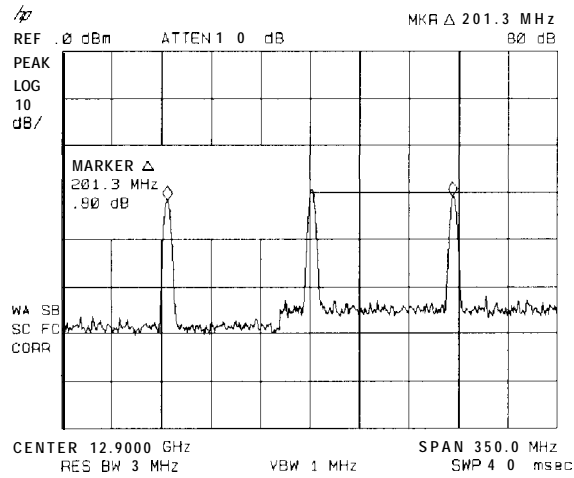
Figure 3-29. Harmonic Locking Off
