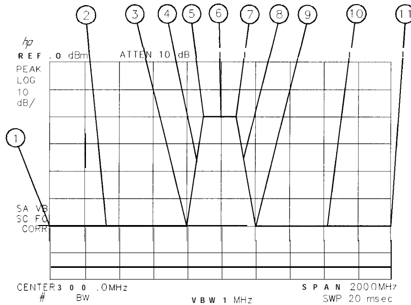
Figure 5-6. Limit-Line Segments
