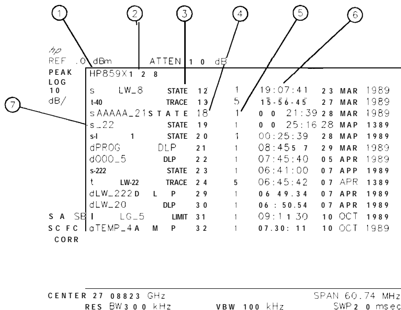
Figure 7-1. Memory Card Catalog Information
