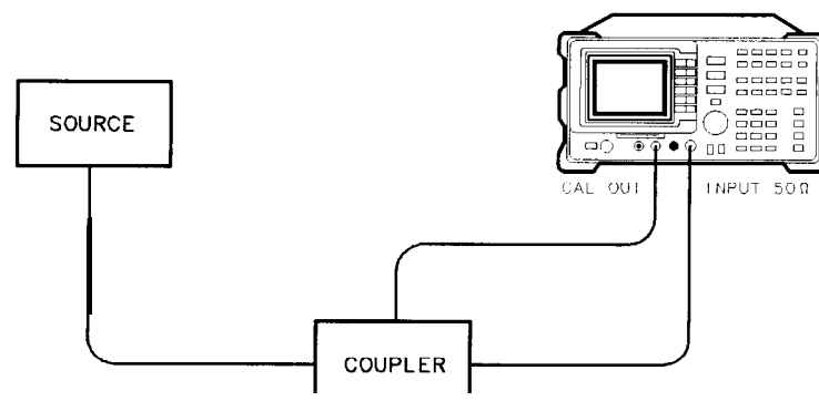
Figure 3-1. Set-Up for Obtaining Two Signals
