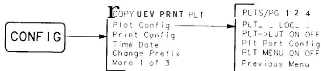
Figure 6-15. Plot Configure Menu
