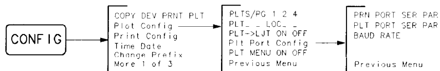
Figure 6-11. Baud Rate Menu Map
