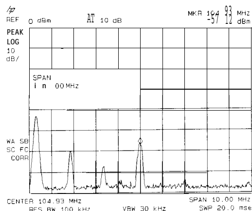
Figure 3-16. Low-Level Signal
