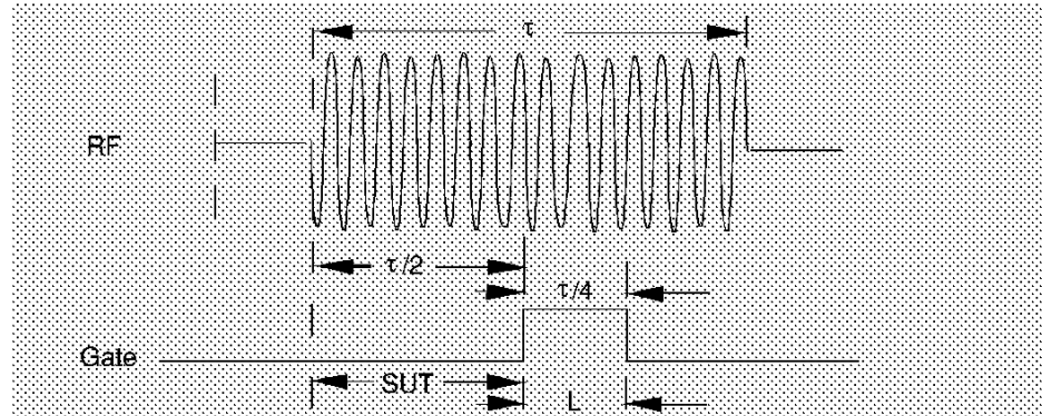
Figure 2-75 Positioning the Gate
