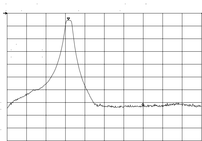
Figure 2-38 Measure the rejection range with delta markers.
