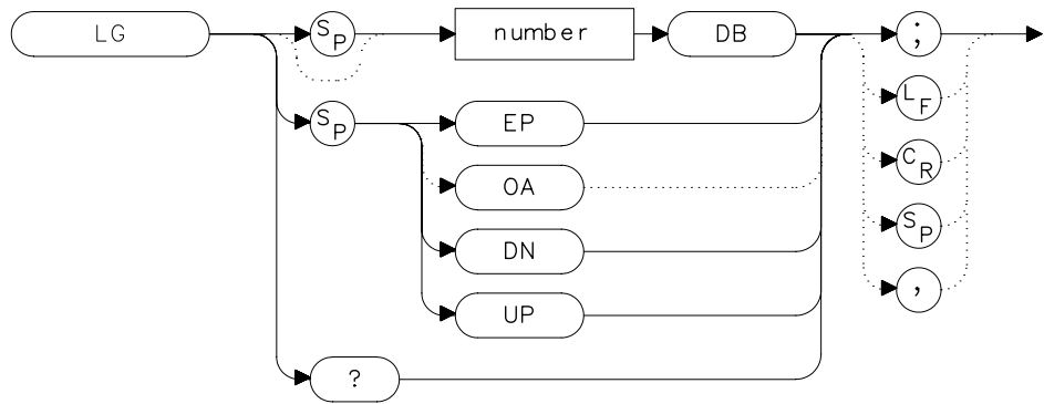
Figure 7-144 LG Syntax
