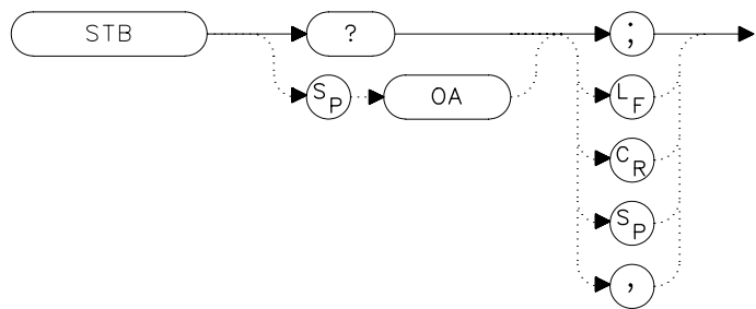
Figure 7-265 STB Syntax
