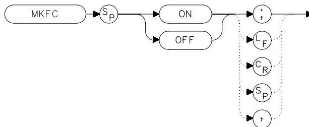
MKFC Syntax
