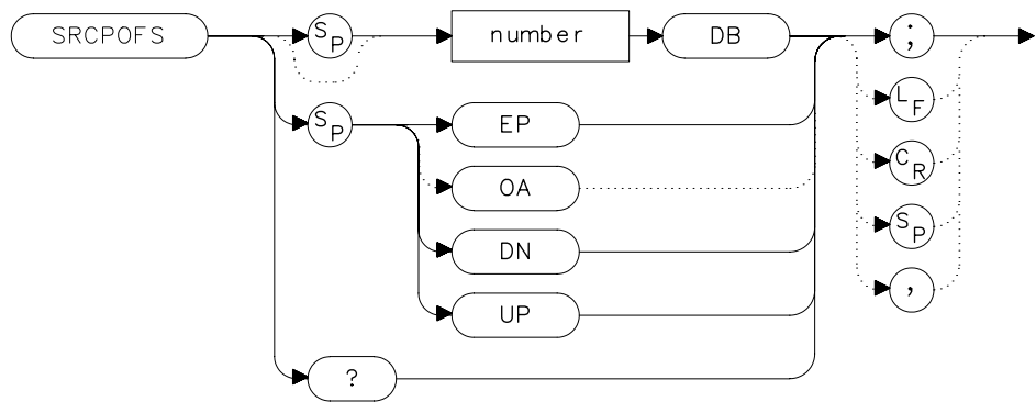
Figure 7-251 SRCPOFS Syntax
