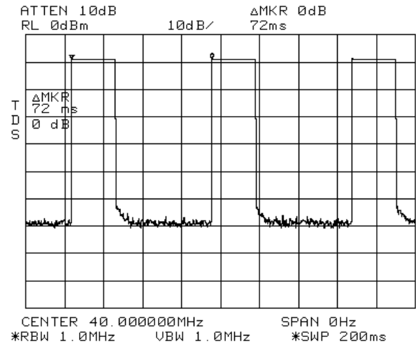
Pulsed-RF Signal in Time Domain
