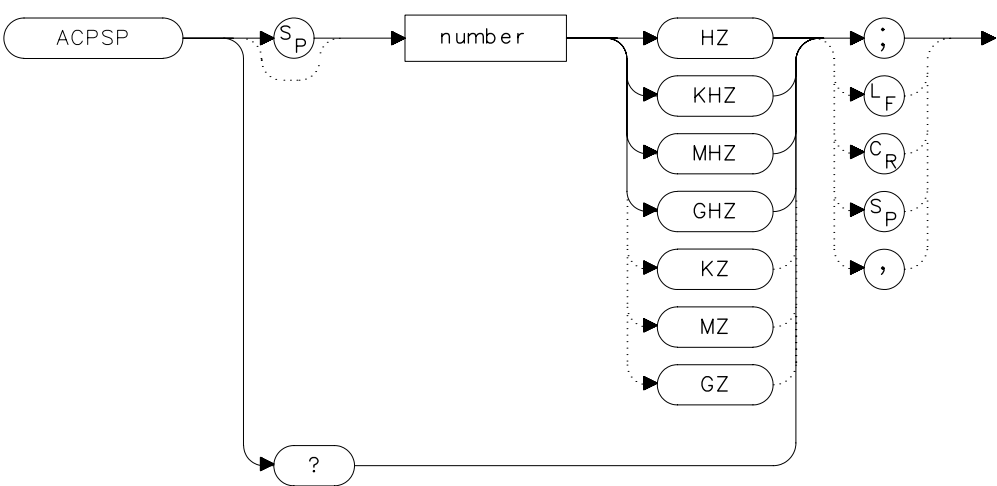
Figure 7-34 ACPSP Syntax
