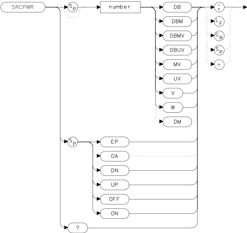
Figure 7-257 SRCPWR Syntax
