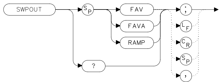
Figure 7-272 SWPOUT Syntax
