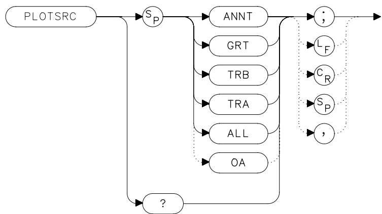
Figure 7-207 PLOTSRC Syntax
