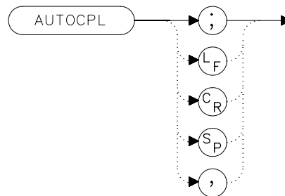
Figure 7-64 AUTOPL Syntax
