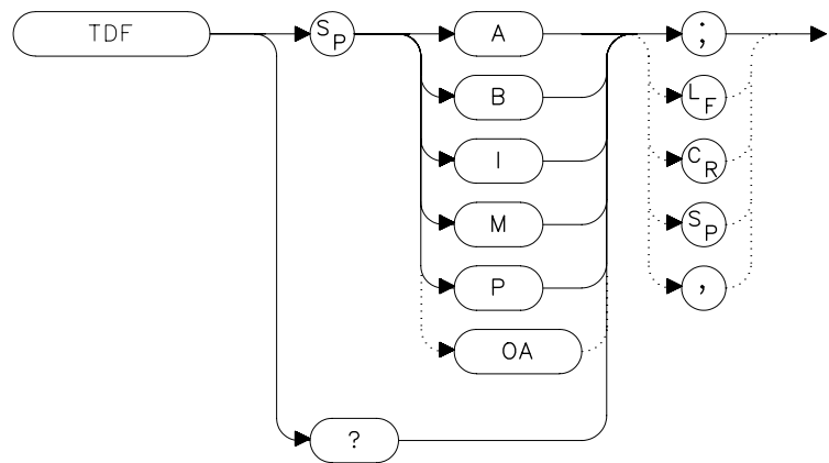
Figure 7-274 TDF Syntax
