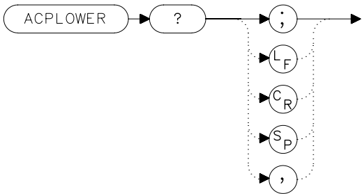
Figure 7-21 ACPLOWER Syntax
