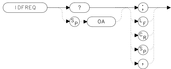
Figure 7-141 IDFREQ Syntax
