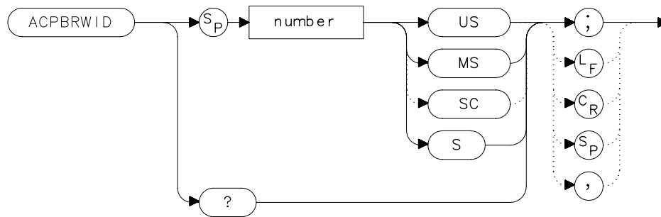
Figure 7-12 ACPBRWID Syntax
