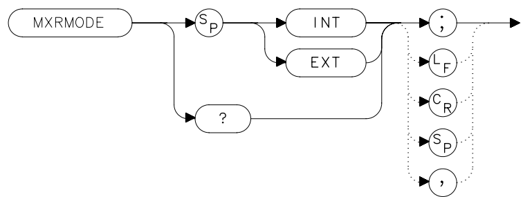
Figure 7-192 MXRMODE Syntax
