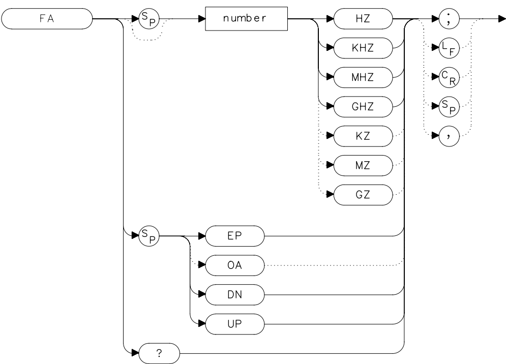
Figure 7-107 FA Syntax
