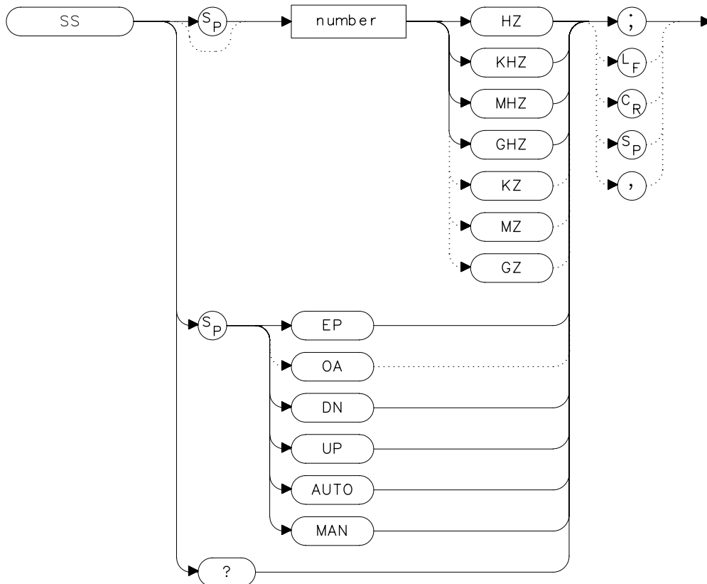
Figure 7-261 SS Syntax
