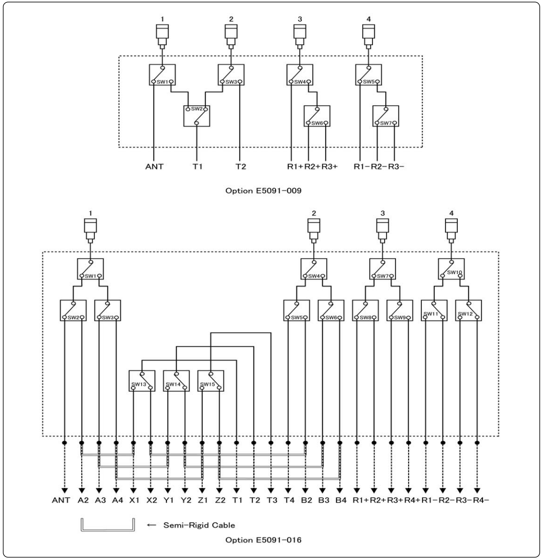
Figure 2-6. Block diagram
