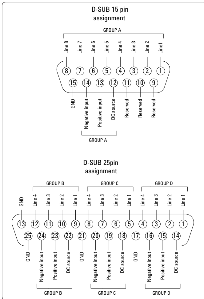
Figure 16. Control line pin assignment (E5092A-020)
